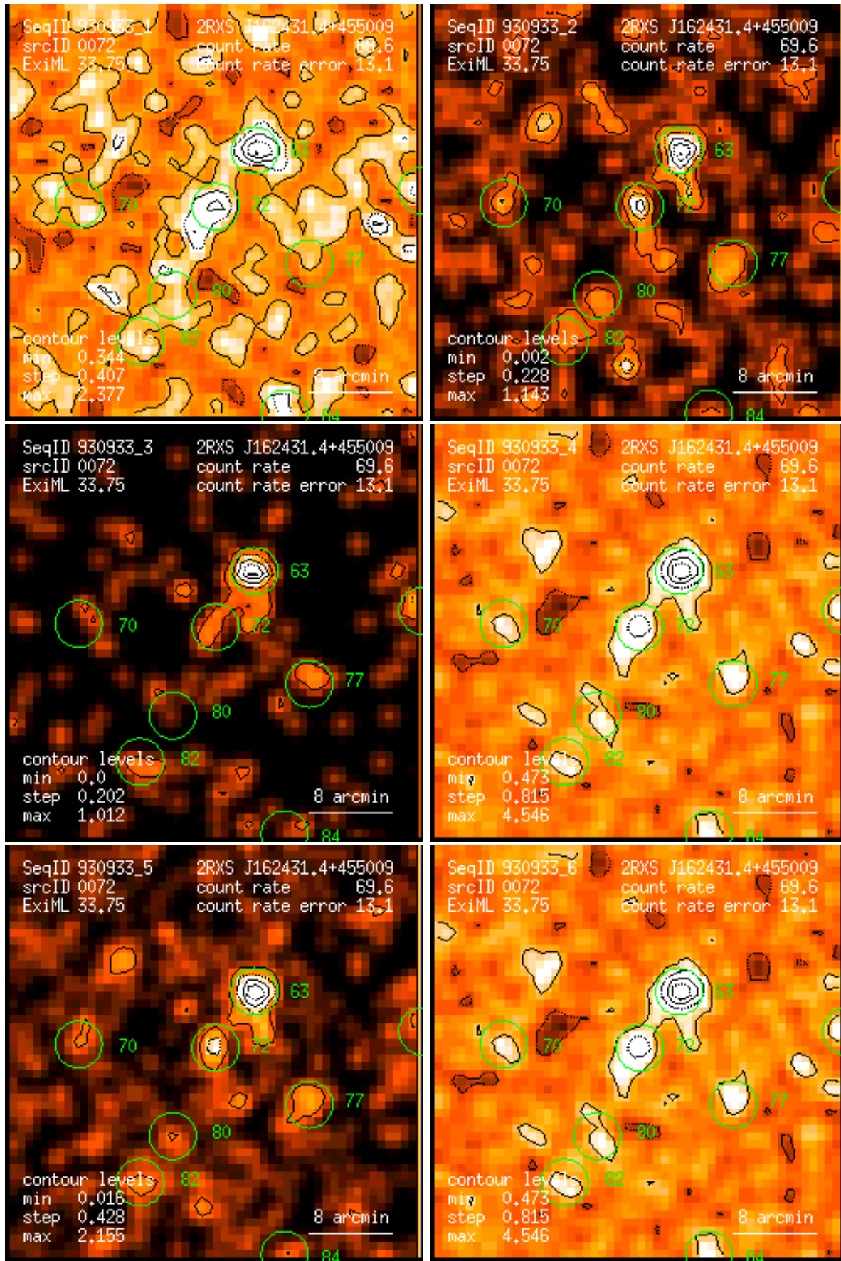
Figure 72: RASS 930933: detection 0072: band rate images, Gaussian filter: (1) PSPC channels 11 – 41, (2) 52 – 90, (3) 91 – 201, (4) 11 – 235, (5) 52 – 201, (6) 11 – 201. Broad band rates in counts/ks. Band rate contour levels in counts/ks/arcmin 2 .
