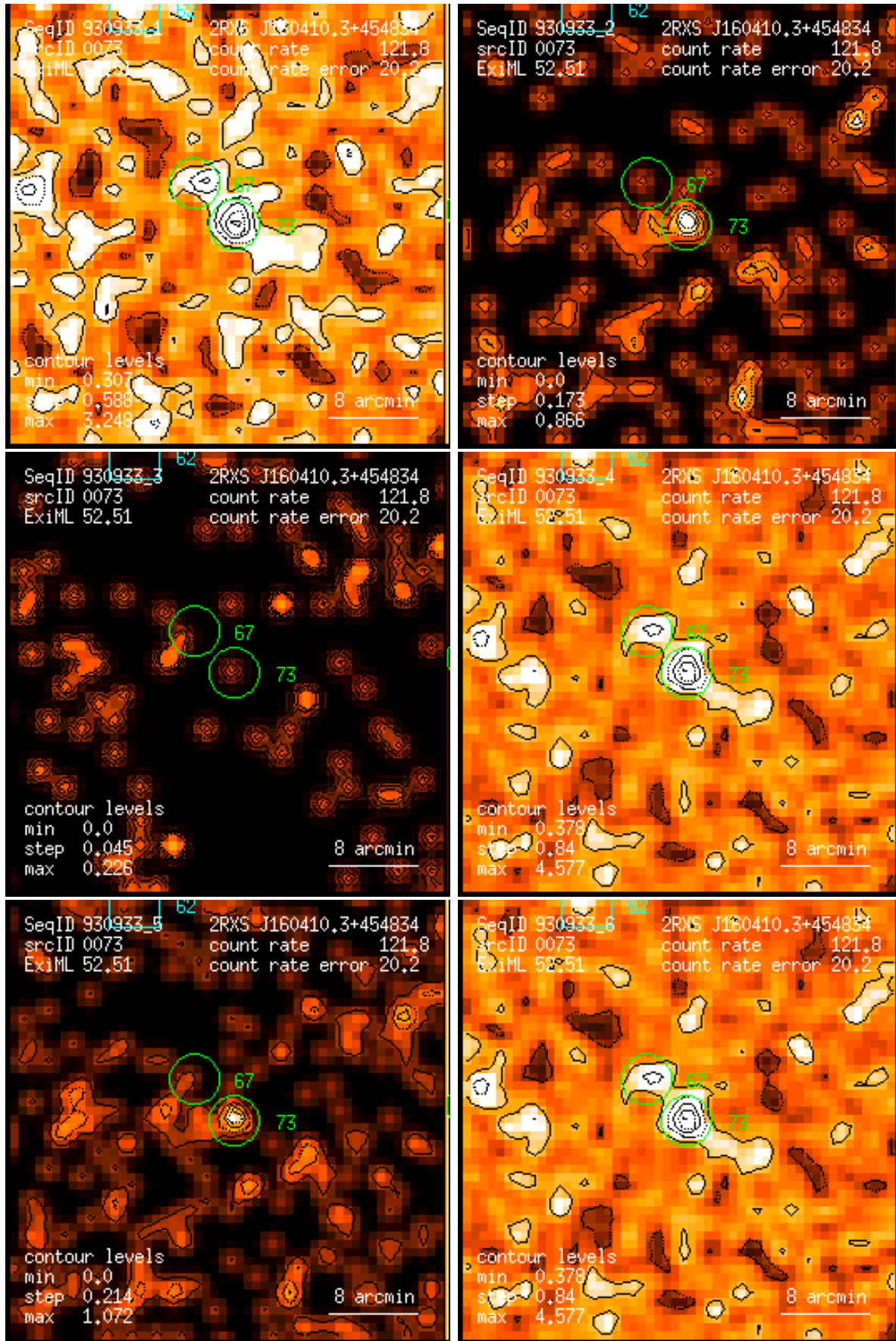
Figure 73: RASS 930933: detection 0073: band rate images, Gaussian filter: (1) PSPC channels 11 – 41, (2) 52 – 90, (3) 91 – 201, (4) 11 – 235, (5) 52 – 201, (6) 11 – 201. Broad band rates in counts/ks. Band rate contour levels in counts/ks/arcmin 2 .
