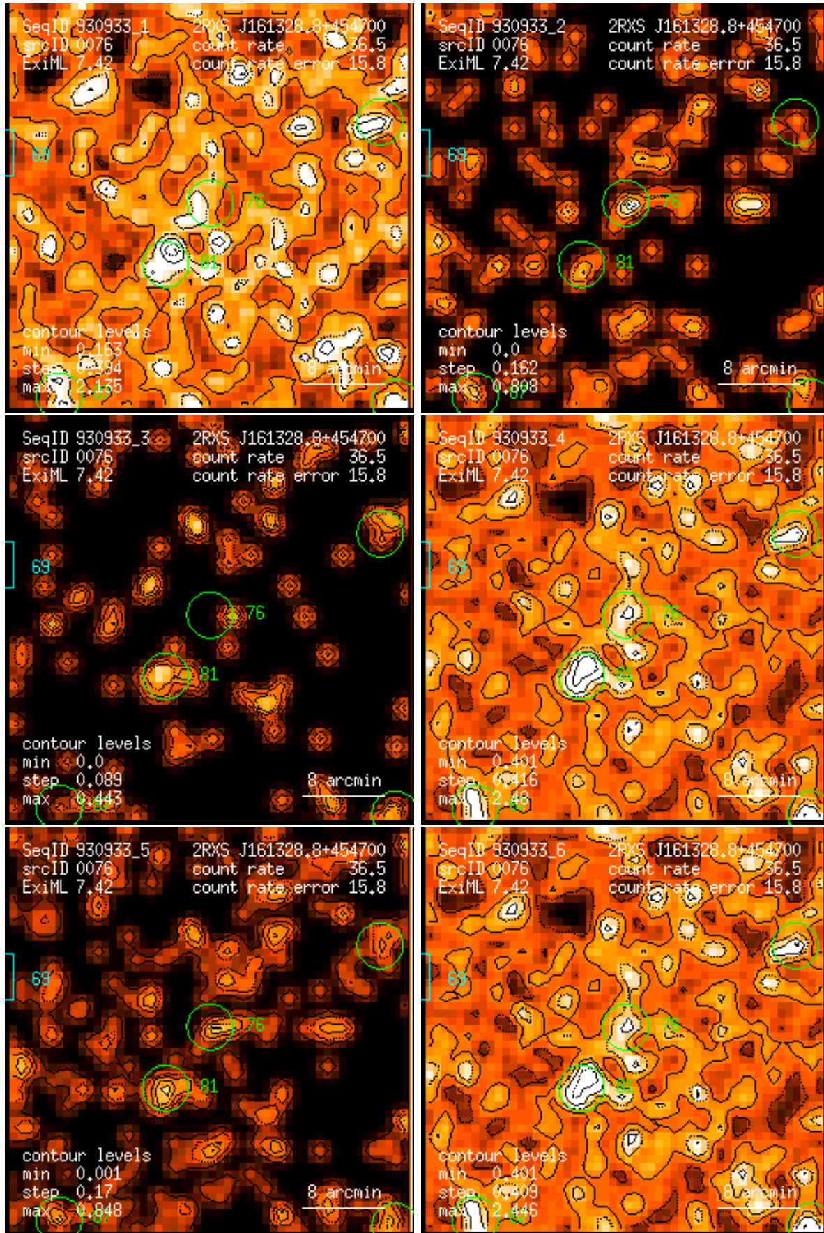
Figure 76: RASS 930933: detection 0076: band rate images, Gaussian filter: (1) PSPC channels 11 – 41, (2) 52 – 90, (3) 91 – 201, (4) 11 – 235, (5) 52 – 201, (6) 11 – 201. Broad band rates in counts/ks. Band rate contour levels in counts/ks/arcmin 2 .
