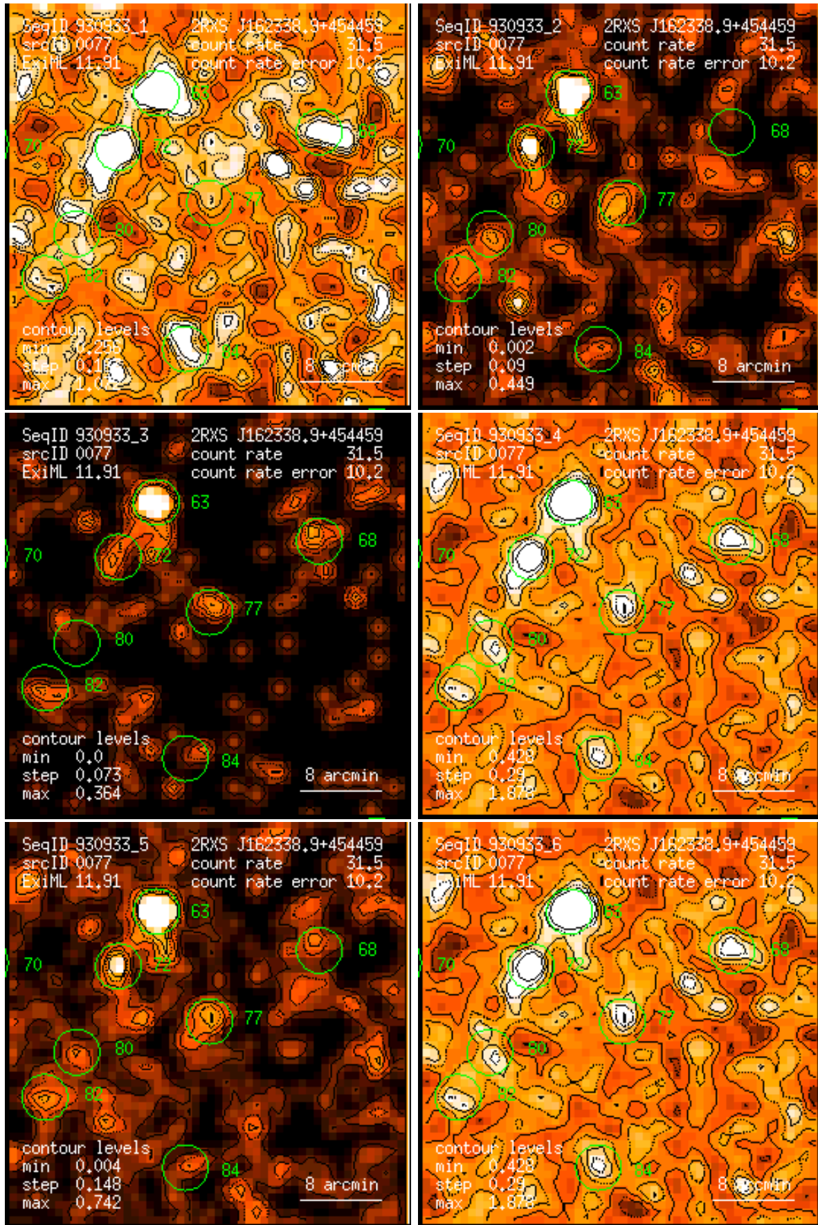
Figure 77: RASS 930933: detection 0077: band rate images, Gaussian filter: (1) PSPC channels 11 – 41, (2) 52 – 90, (3) 91 – 201, (4) 11 – 235, (5) 52 – 201, (6) 11 – 201. Broad band rates in counts/ks. Band rate contour levels in counts/ks/arcmin 2 .
