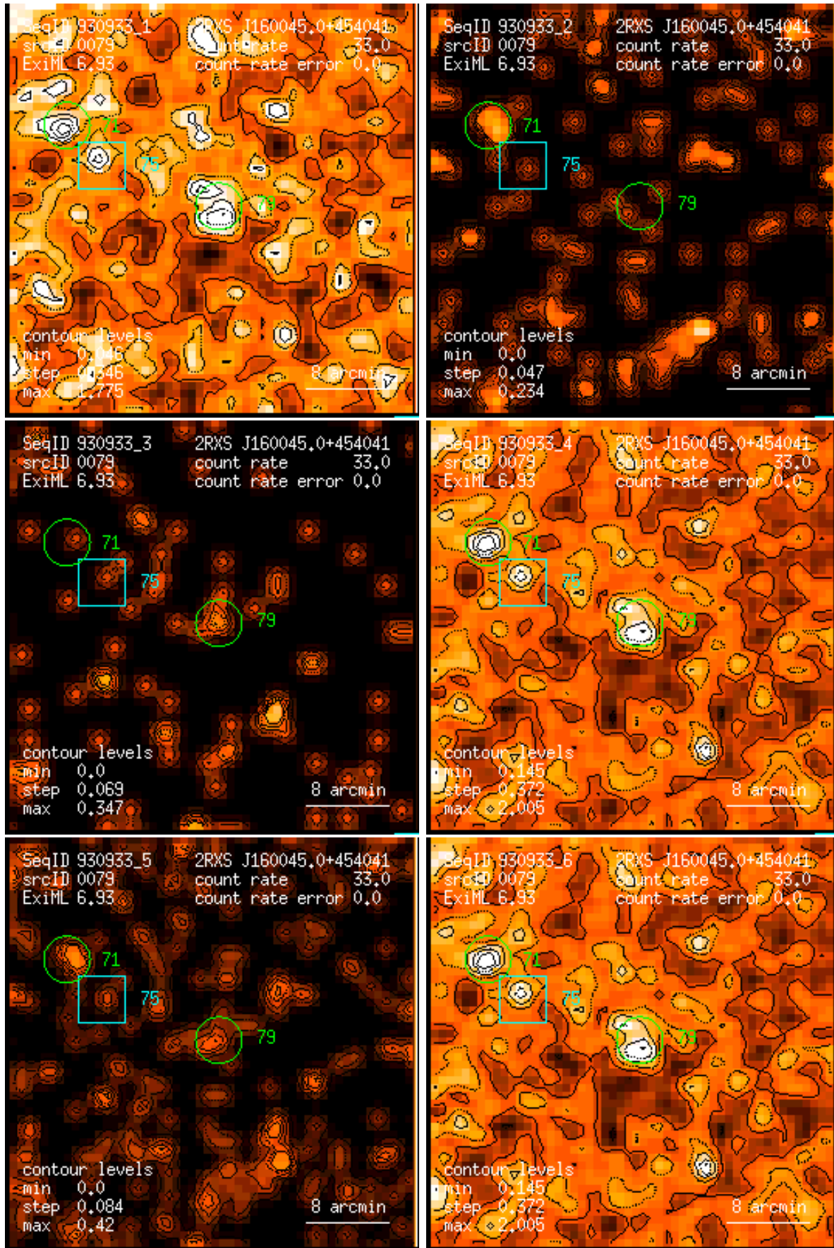
Figure 79: RASS 930933: detection 0079: band rate images, Gaussian filter: (1) PSPC channels 11 – 41, (2) 52 – 90, (3) 91 – 201, (4) 11 – 235, (5) 52 – 201, (6) 11 – 201. Broad band rates in counts/ks. Band rate contour levels in counts/ks/arcmin 2 .
