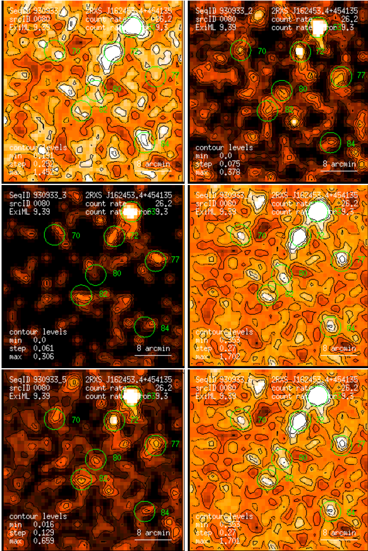
Figure 80: RASS 930933: detection 0080: band rate images, Gaussian filter: (1) PSPC channels 11 – 41, (2) 52 – 90, (3) 91 – 201, (4) 11 – 235, (5) 52 – 201, (6) 11 – 201. Broad band rates in counts/ks. Band rate contour levels in counts/ks/arcmin 2 .
