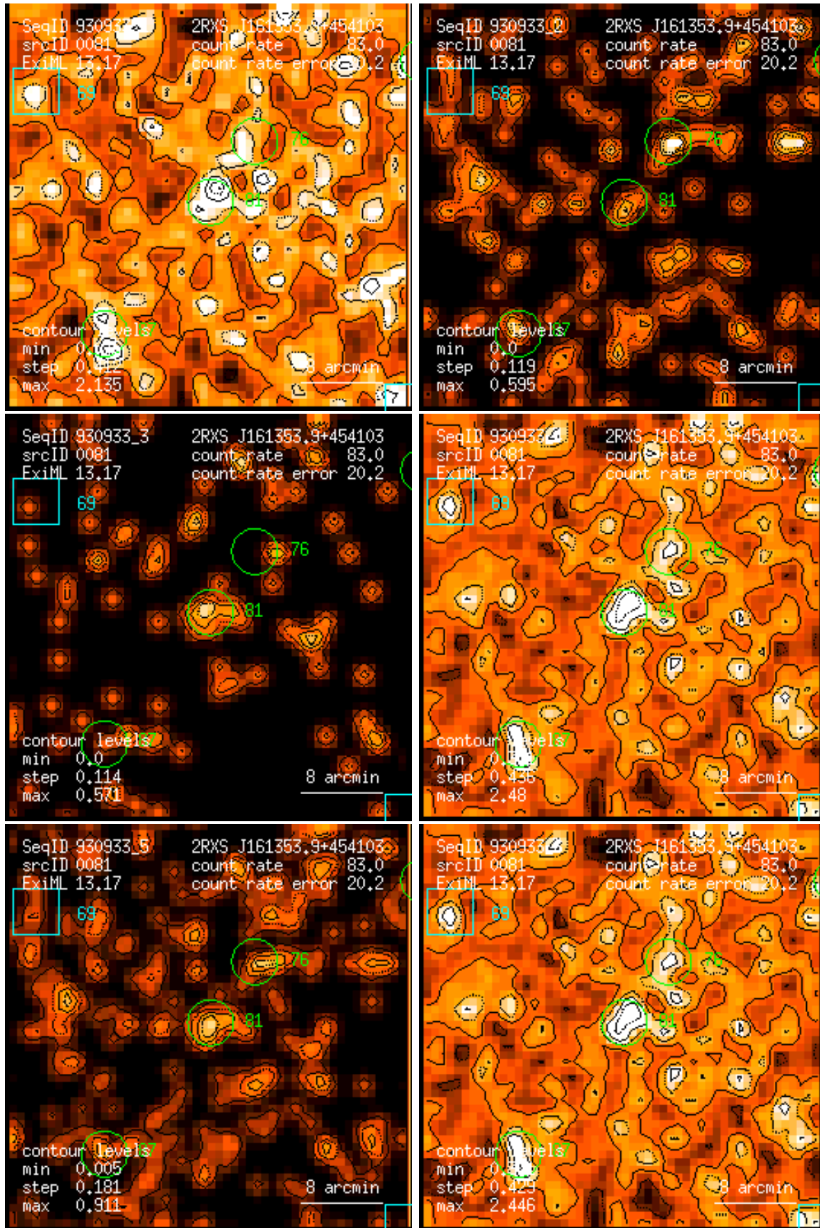
Figure 81: RASS 930933: detection 0081: band rate images, Gaussian filter: (1) PSPC channels 11 – 41, (2) 52 – 90, (3) 91 – 201, (4) 11 – 235, (5) 52 – 201, (6) 11 – 201. Broad band rates in counts/ks. Band rate contour levels in counts/ks/arcmin 2 .
