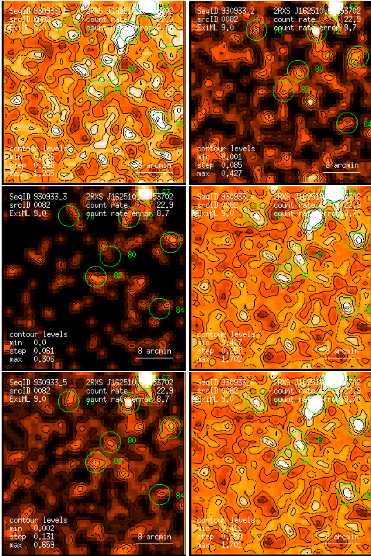
Figure 82: RASS 930933: detection 0082: band rate images, Gaussian filter: (1) PSPC channels 11 – 41, (2) 52 – 90, (3) 91 – 201, (4) 11 – 235, (5) 52 – 201, (6) 11 – 201. Broad band rates in counts/ks. Band rate contour levels in counts/ks/arcmin 2 .
