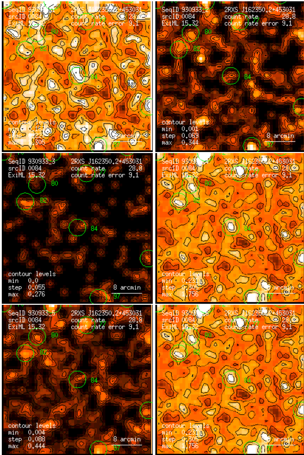
Figure 84: RASS 930933: detection 0084: band rate images, Gaussian filter: (1) PSPC channels 11 – 41, (2) 52 – 90, (3) 91 – 201, (4) 11 – 235, (5) 52 – 201, (6) 11 – 201. Broad band rates in counts/ks. Band rate contour levels in counts/ks/arcmin 2 .
