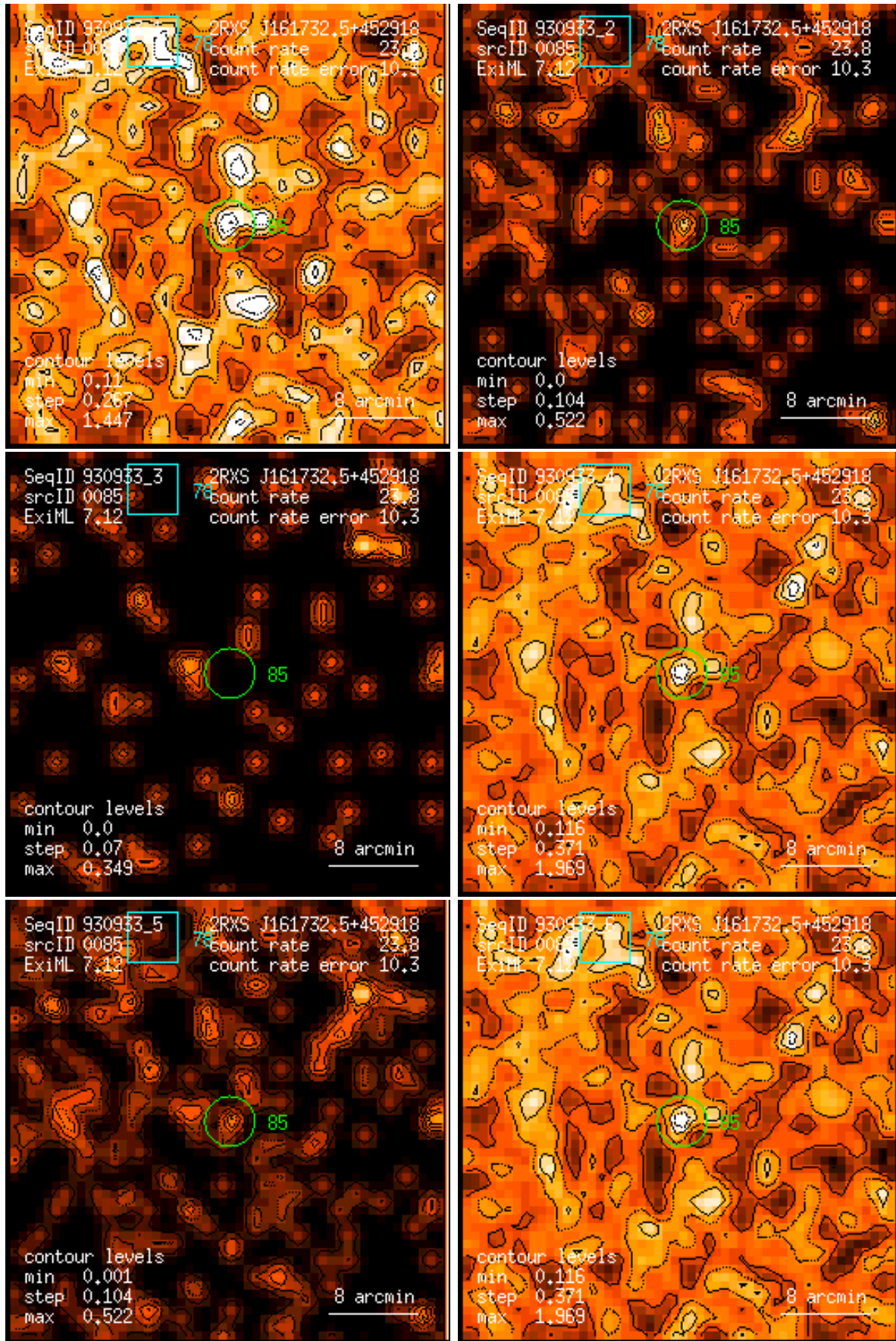
Figure 85: RASS 930933: detection 0085: band rate images, Gaussian filter: (1) PSPC channels 11 – 41, (2) 52 – 90, (3) 91 – 201, (4) 11 – 235, (5) 52 – 201, (6) 11 – 201. Broad band rates in counts/ks. Band rate contour levels in counts/ks/arcmin 2 .
