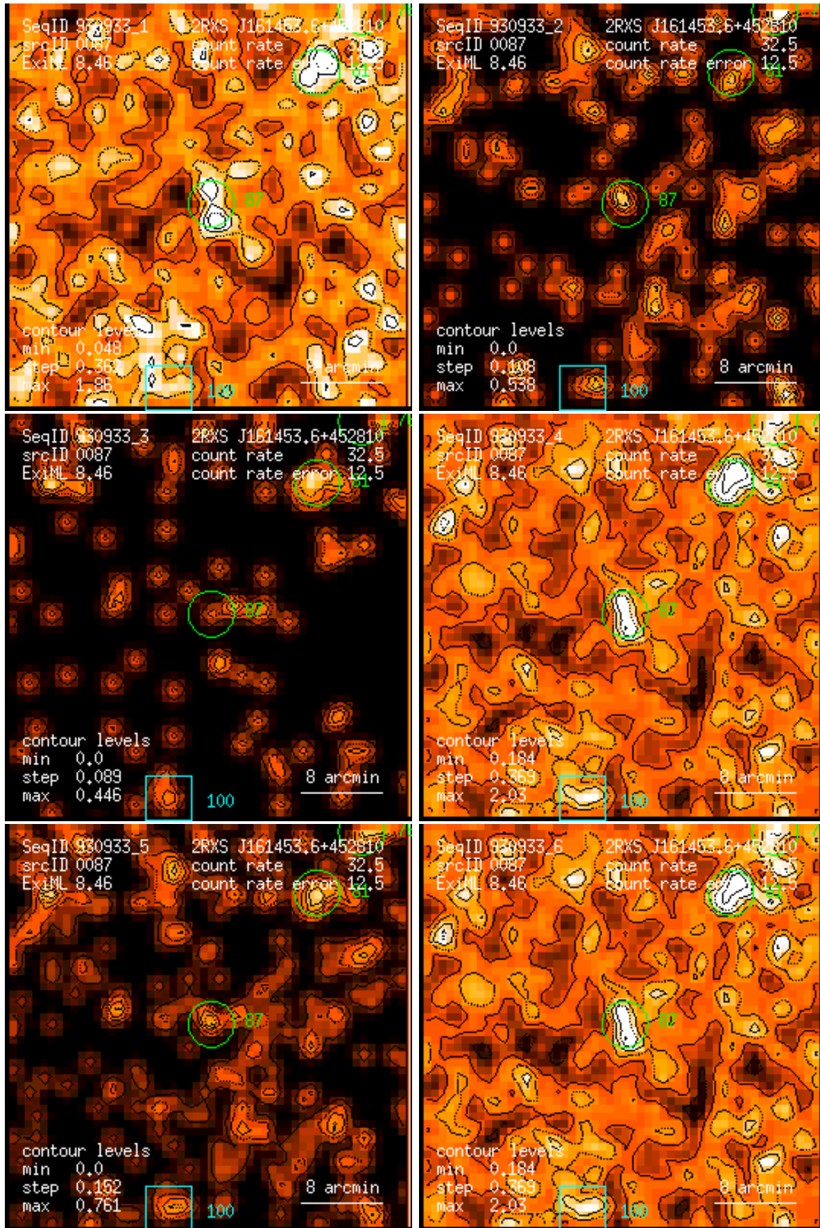
Figure 87: RASS 930933: detection 0087: band rate images, Gaussian filter: (1) PSPC channels 11 – 41, (2) 52 – 90, (3) 91 – 201, (4) 11 – 235, (5) 52 – 201, (6) 11 – 201. Broad band rates in counts/ks. Band rate contour levels in counts/ks/arcmin 2 .
