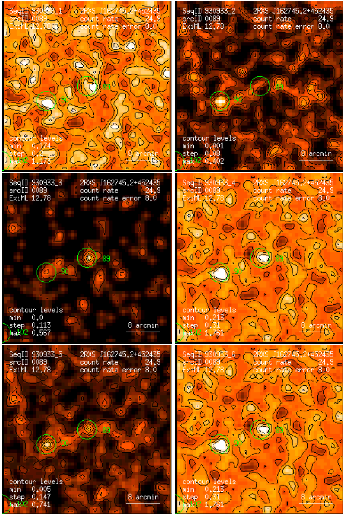
Figure 89: RASS 930933: detection 0089: band rate images, Gaussian filter: (1) PSPC channels 11 – 41, (2) 52 – 90, (3) 91 – 201, (4) 11 – 235, (5) 52 – 201, (6) 11 – 201. Broad band rates in counts/ks. Band rate contour levels in counts/ks/arcmin 2 .
