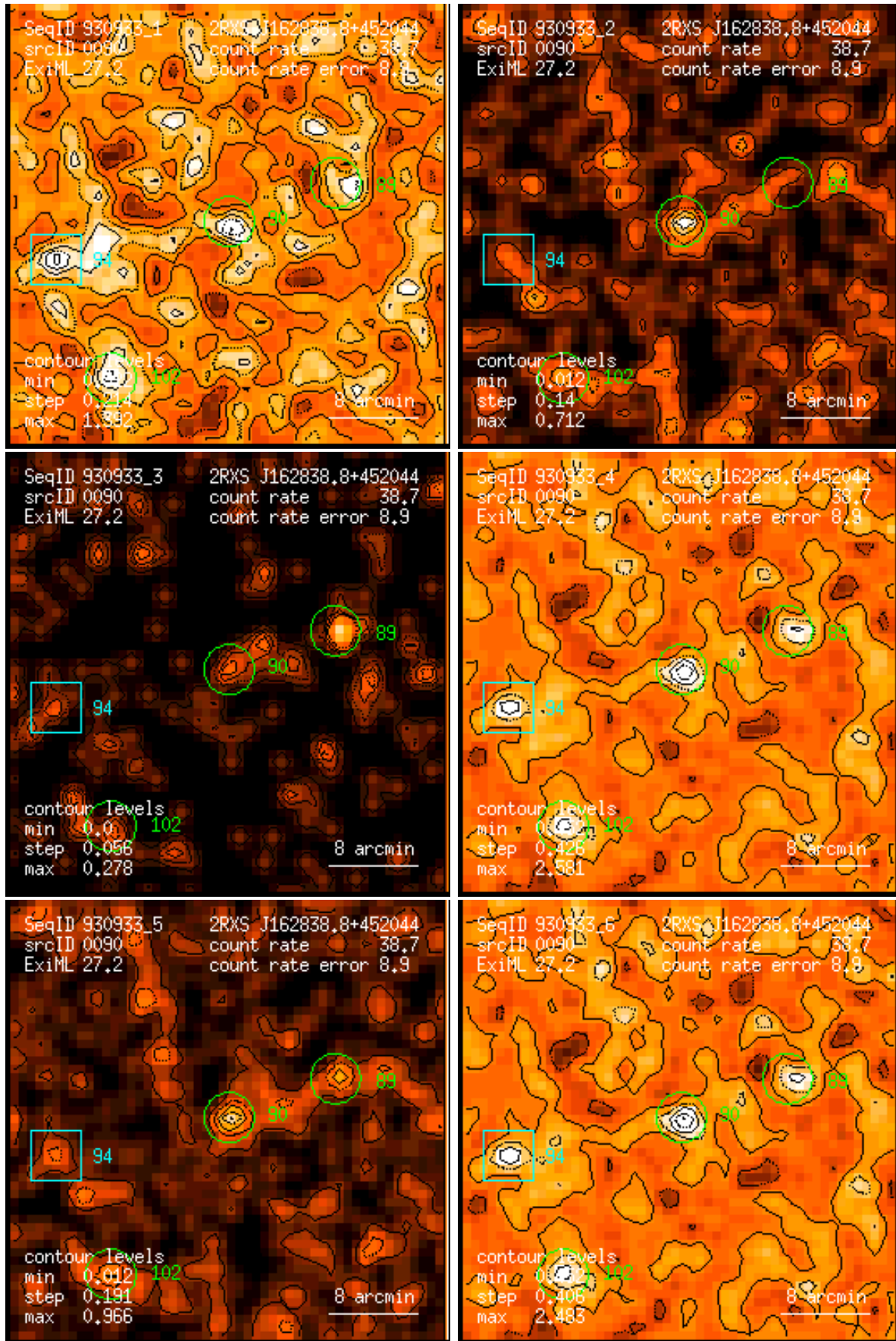
Figure 90: RASS 930933: detection 0090: band rate images, Gaussian filter: (1) PSPC channels 11 – 41, (2) 52 – 90, (3) 91 – 201, (4) 11 – 235, (5) 52 – 201, (6) 11 – 201. Broad band rates in counts/ks. Band rate contour levels in counts/ks/arcmin 2 .
