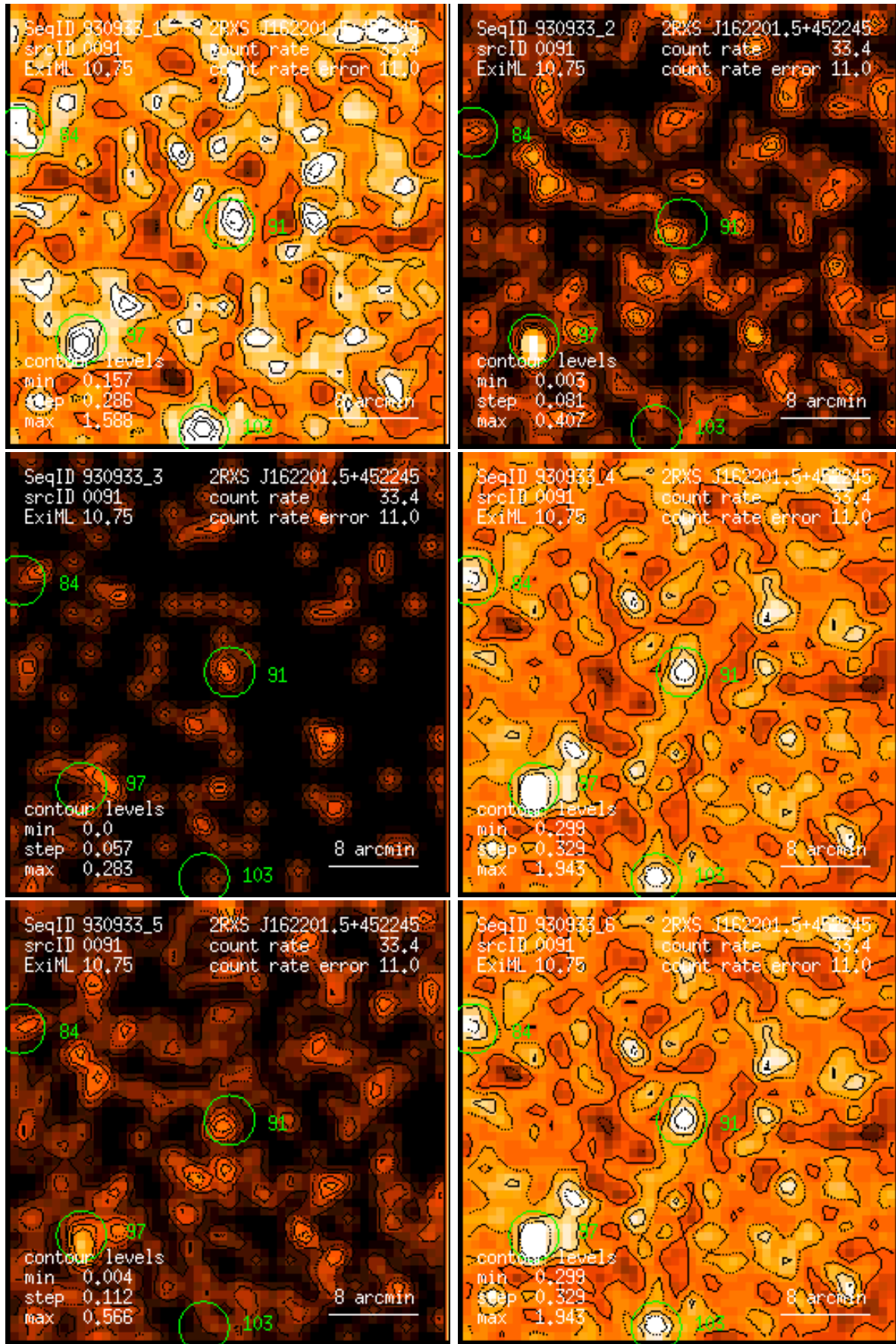
Figure 91: RASS 930933: detection 0091: band rate images, Gaussian filter: (1) PSPC channels 11 – 41, (2) 52 – 90, (3) 91 – 201, (4) 11 – 235, (5) 52 – 201, (6) 11 – 201. Broad band rates in counts/ks. Band rate contour levels in counts/ks/arcmin 2 .
