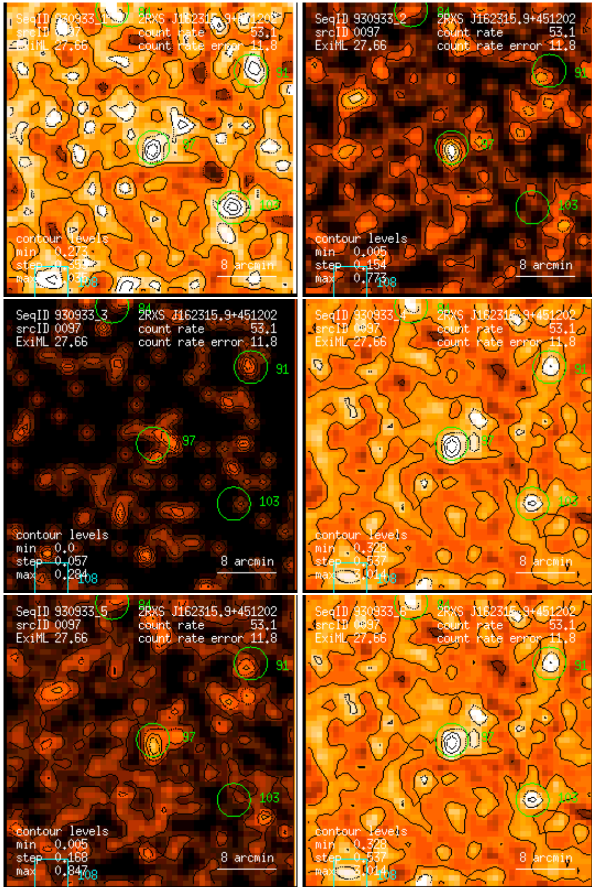
Figure 97: RASS 930933: detection 0097: band rate images, Gaussian filter: (1) PSPC channels 11 – 41, (2) 52 – 90, (3) 91 – 201, (4) 11 – 235, (5) 52 – 201, (6) 11 – 201. Broad band rates in counts/ks. Band rate contour levels in counts/ks/arcmin 2 .
