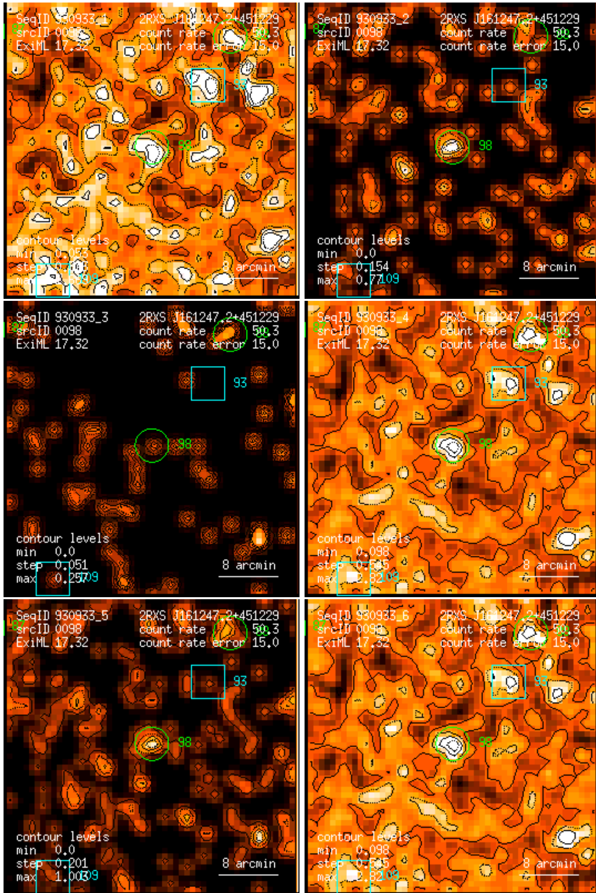
Figure 98: RASS 930933: detection 0098: band rate images, Gaussian filter: (1) PSPC channels 11 – 41, (2) 52 – 90, (3) 91 – 201, (4) 11 – 235, (5) 52 – 201, (6) 11 – 201. Broad band rates in counts/ks. Band rate contour levels in counts/ks/arcmin 2 .
