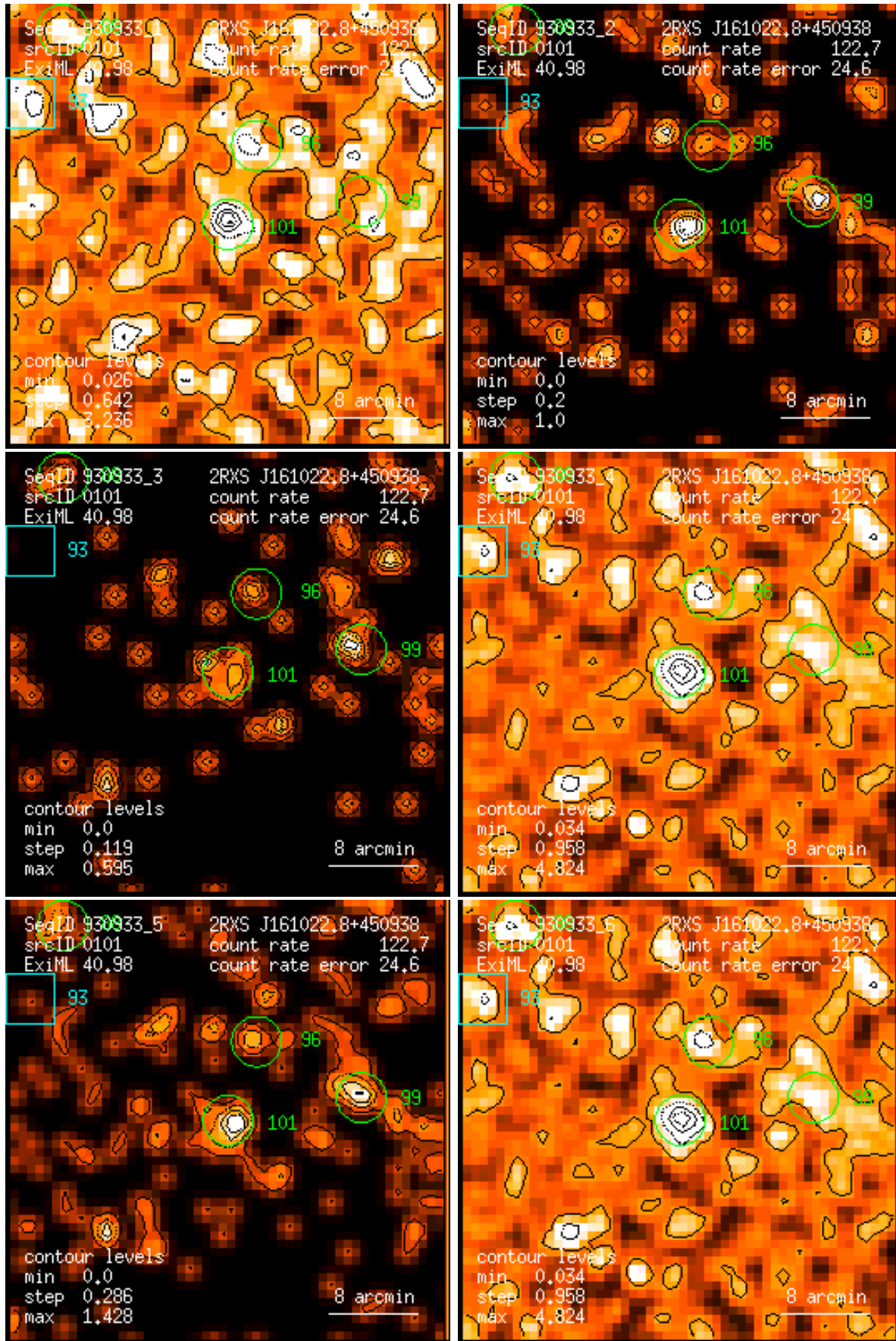
Figure 101: RASS 930933: detection 0101: band rate images, Gaussian filter: (1) PSPC channels 11 – 41, (2) 52 – 90, (3) 91 – 201, (4) 11 – 235, (5) 52 – 201, (6) 11 – 201. Broad band rates in counts/ks. Band rate contour levels in counts/ks/arcmin 2 .
