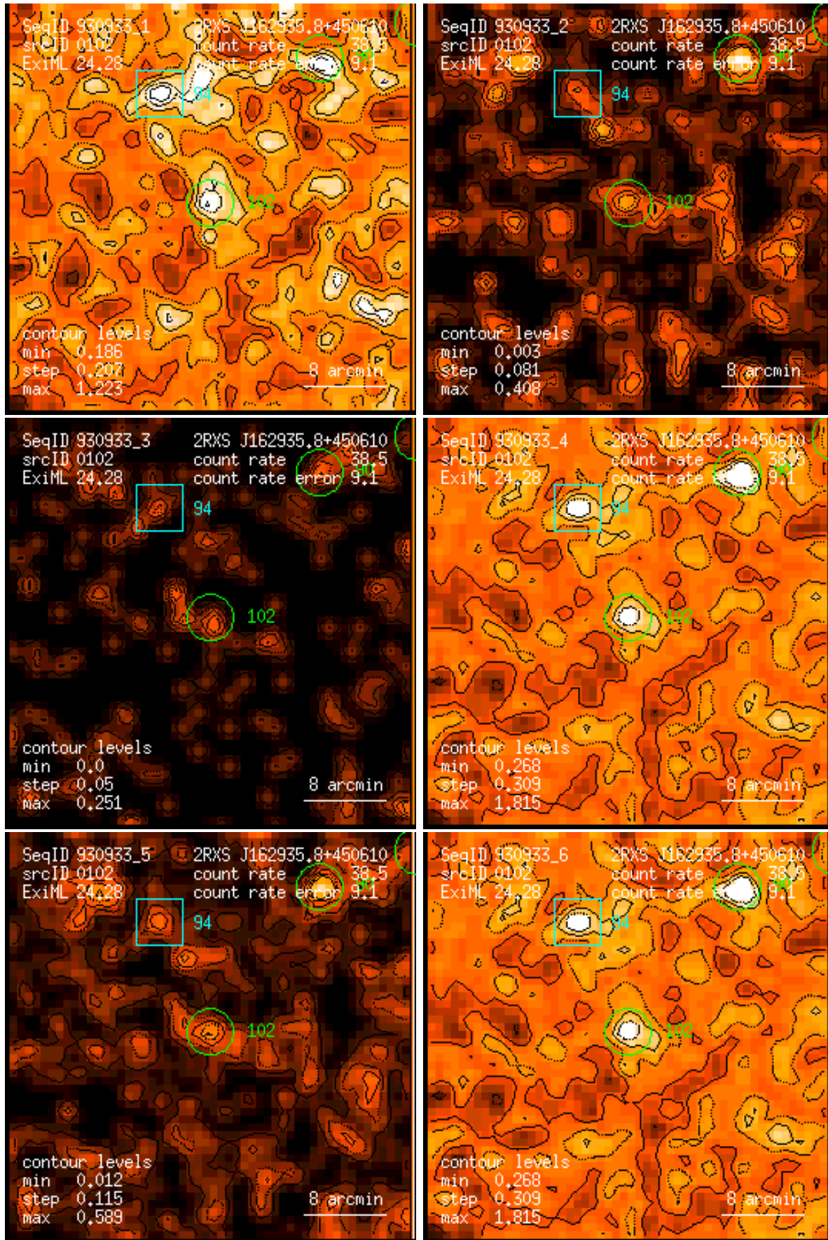
Figure 102: RASS 930933: detection 0102: band rate images, Gaussian filter: (1) PSPC channels 11 – 41, (2) 52 – 90, (3) 91 – 201, (4) 11 – 235, (5) 52 – 201, (6) 11 – 201. Broad band rates in counts/ks. Band rate contour levels in counts/ks/arcmin 2 .
