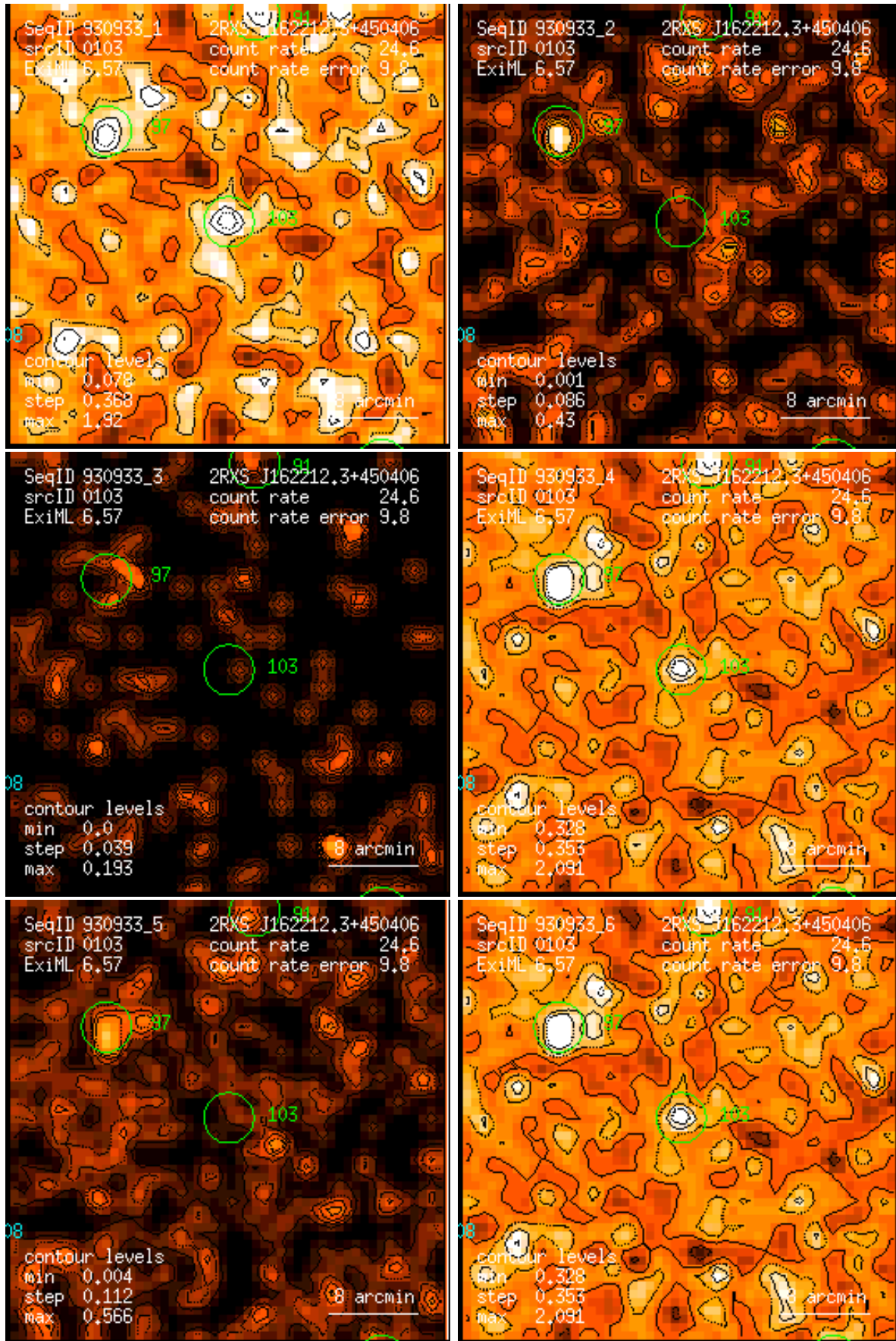
Figure 103: RASS 930933: detection 0103: band rate images, Gaussian filter: (1) PSPC channels 11 – 41, (2) 52 – 90, (3) 91 – 201, (4) 11 – 235, (5) 52 – 201, (6) 11 – 201. Broad band rates in counts/ks. Band rate contour levels in counts/ks/arcmin 2 .
