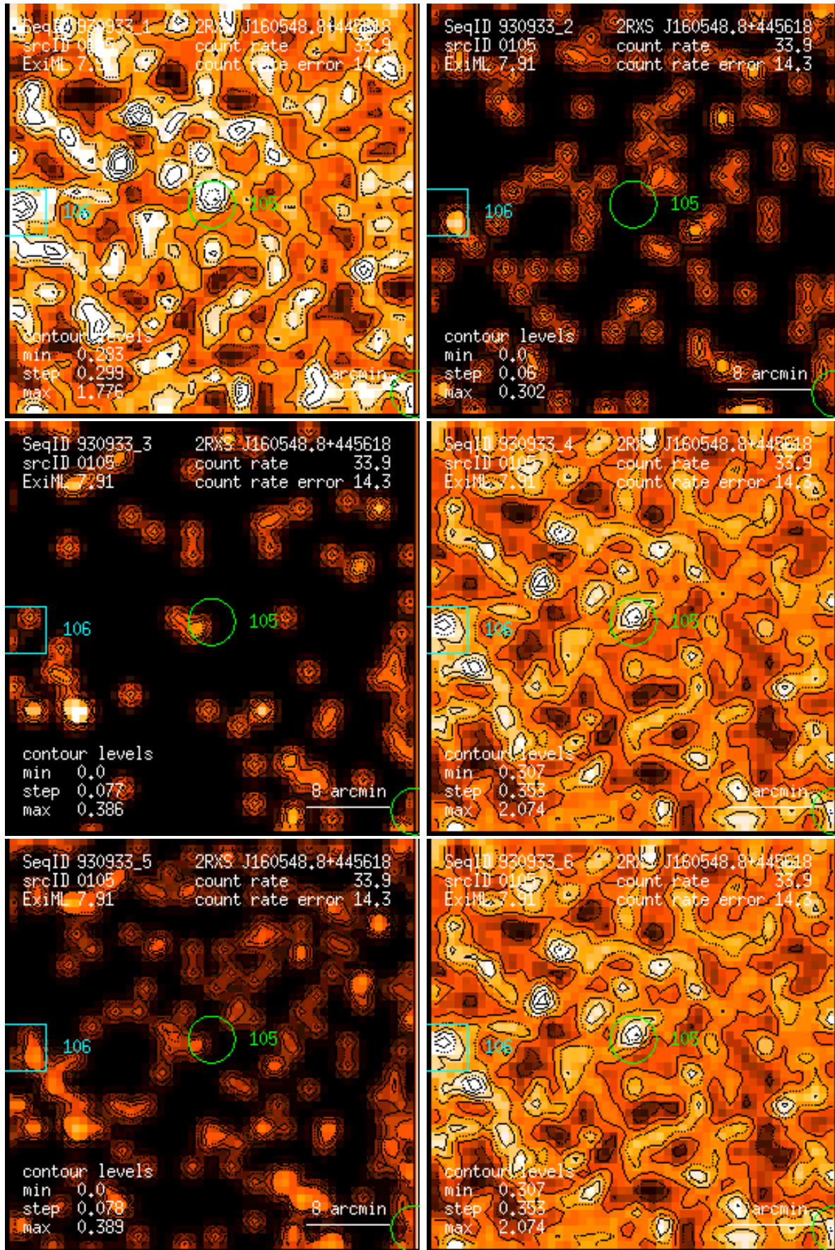
Figure 105: RASS 930933: detection 0105: band rate images, Gaussian filter: (1) PSPC channels 11 – 41, (2) 52 – 90, (3) 91 – 201, (4) 11 – 235, (5) 52 – 201, (6) 11 – 201. Broad band rates in counts/ks. Band rate contour levels in counts/ks/arcmin 2 .
