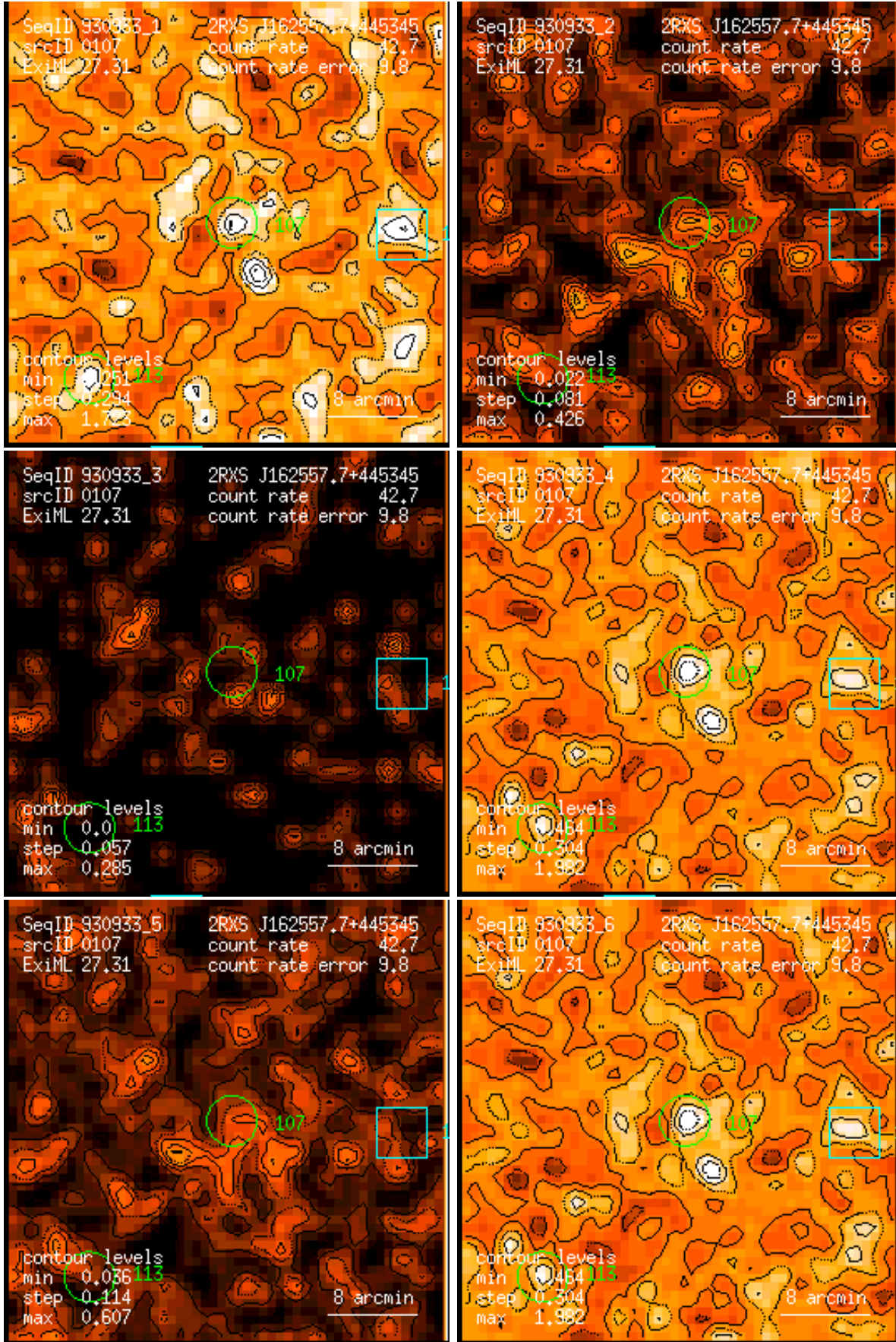
Figure 107: RASS 930933: detection 0107: band rate images, Gaussian filter: (1) PSPC channels 11 – 41, (2) 52 – 90, (3) 91 – 201, (4) 11 – 235, (5) 52 – 201, (6) 11 – 201. Broad band rates in counts/ks. Band rate contour levels in counts/ks/arcmin 2 .
