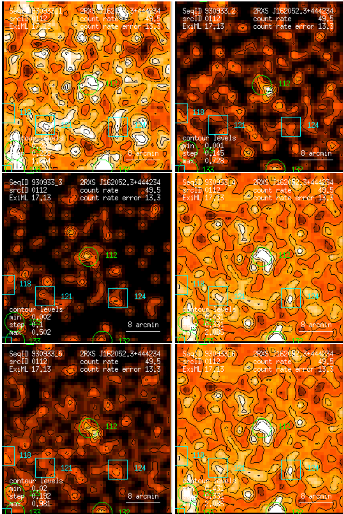
Figure 112: RASS 930933: detection 0112: band rate images, Gaussian filter: (1) PSPC channels 11 – 41, (2) 52 – 90, (3) 91 – 201, (4) 11 – 235, (5) 52 – 201, (6) 11 – 201. Broad band rates in counts/ks. Band rate contour levels in counts/ks/arcmin 2 .
