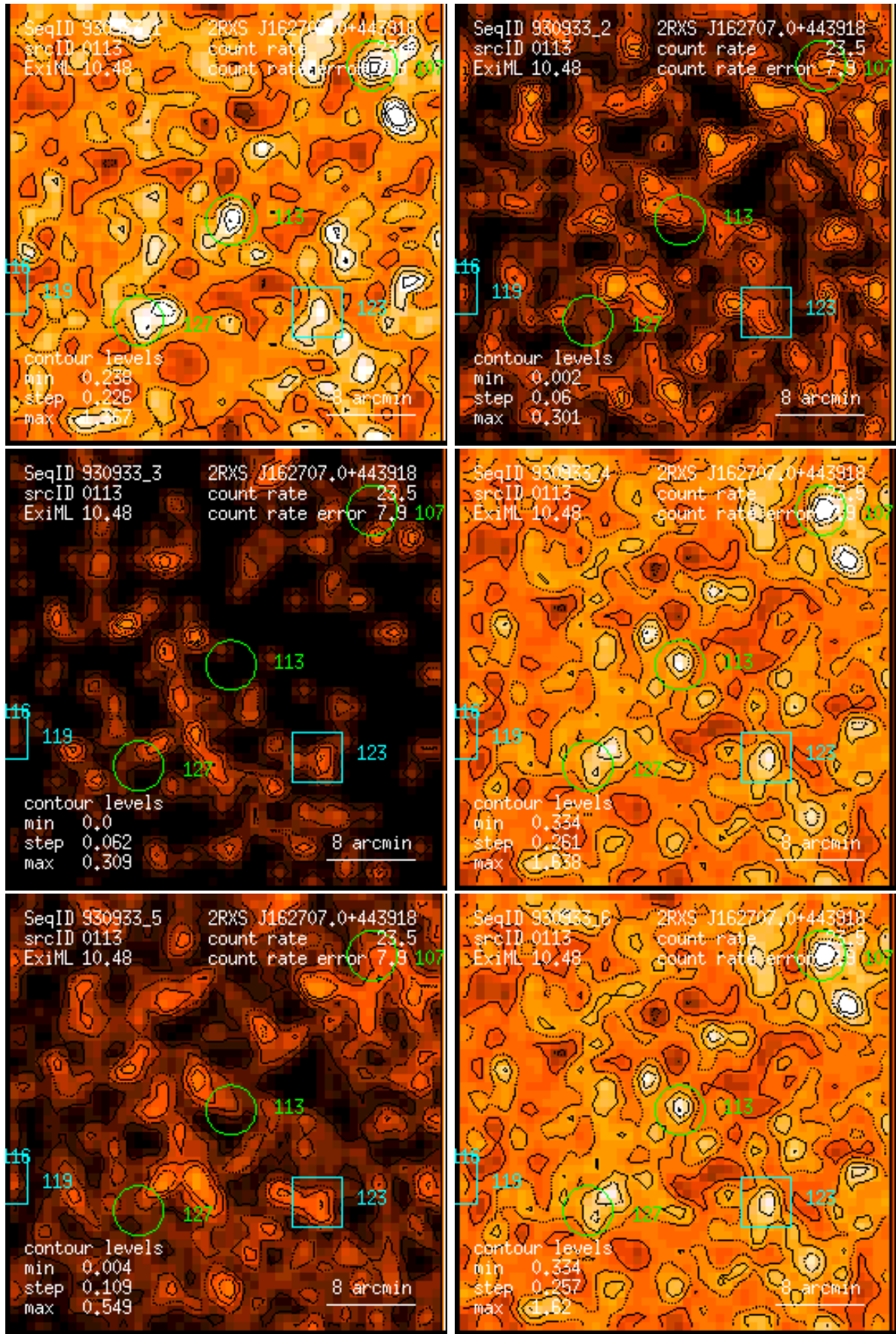
Figure 113: RASS 930933: detection 0113: band rate images, Gaussian filter: (1) PSPC channels 11 – 41, (2) 52 – 90, (3) 91 – 201, (4) 11 – 235, (5) 52 – 201, (6) 11 – 201. Broad band rates in counts/ks. Band rate contour levels in counts/ks/arcmin 2 .
