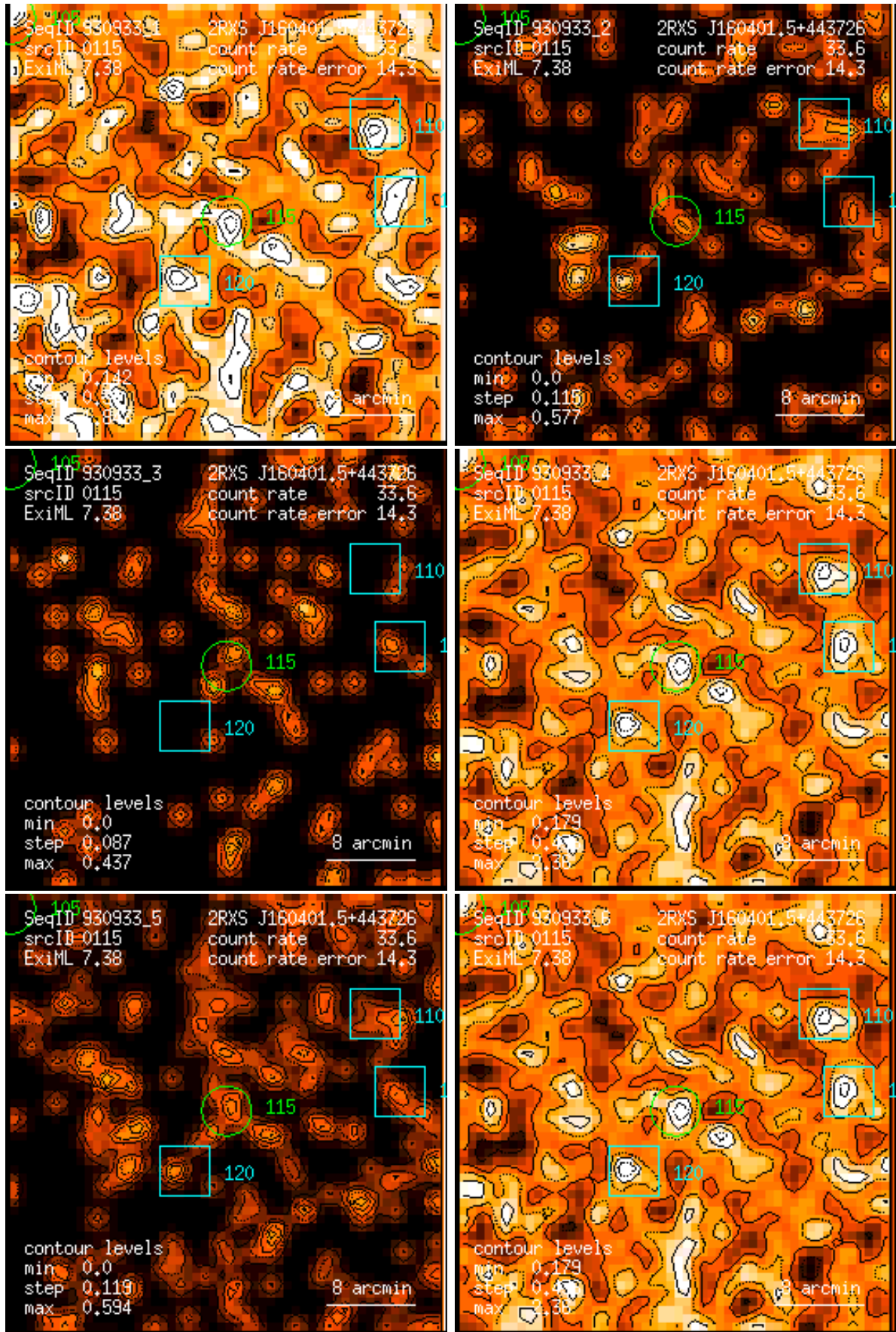
Figure 115: RASS 930933: detection 0115: band rate images, Gaussian filter: (1) PSPC channels 11 – 41, (2) 52 – 90, (3) 91 – 201, (4) 11 – 235, (5) 52 – 201, (6) 11 – 201. Broad band rates in counts/ks. Band rate contour levels in counts/ks/arcmin 2 .
