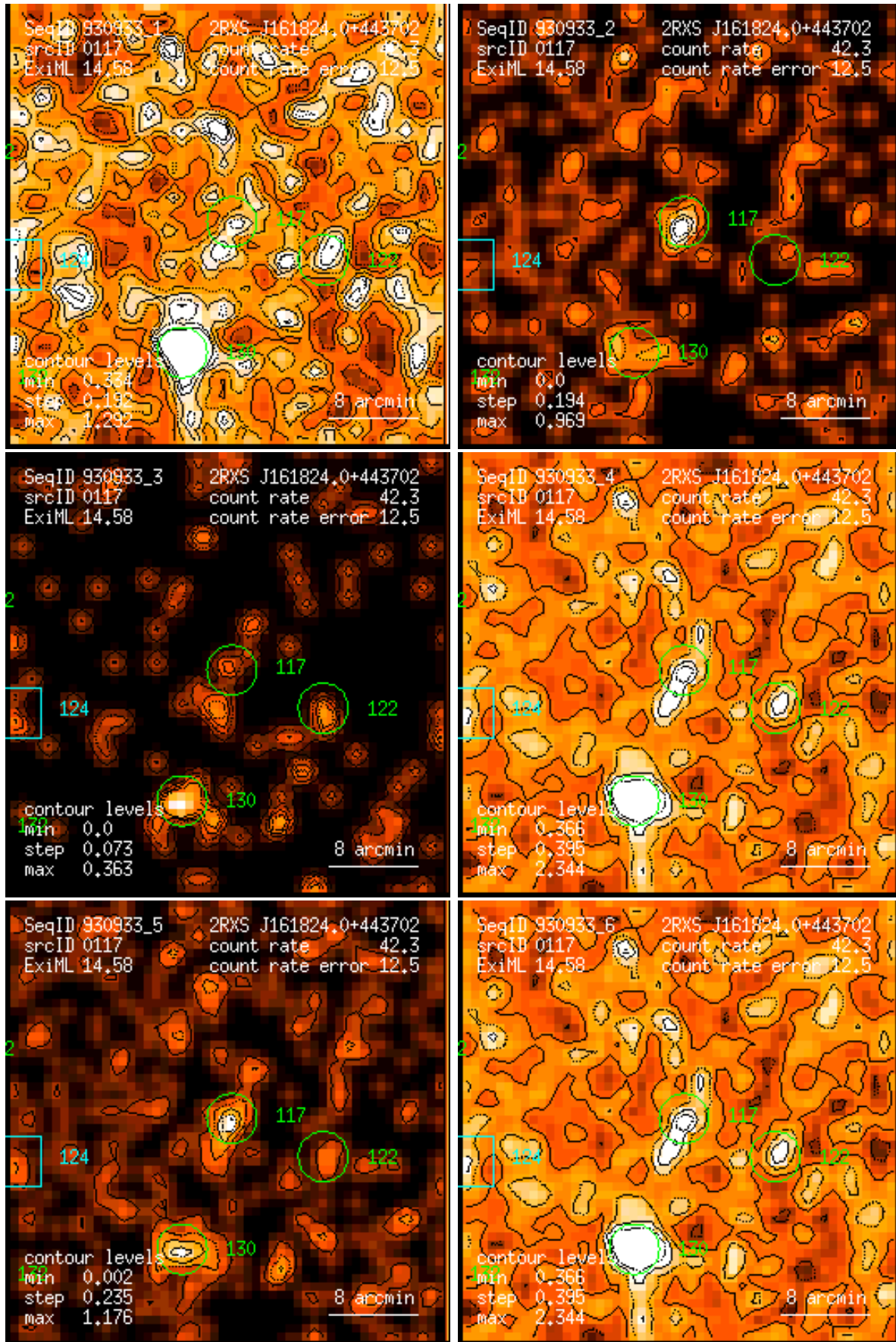
Figure 117: RASS 930933: detection 0117: band rate images, Gaussian filter: (1) PSPC channels 11 – 41, (2) 52 – 90, (3) 91 – 201, (4) 11 – 235, (5) 52 – 201, (6) 11 – 201. Broad band rates in counts/ks. Band rate contour levels in counts/ks/arcmin 2 .
