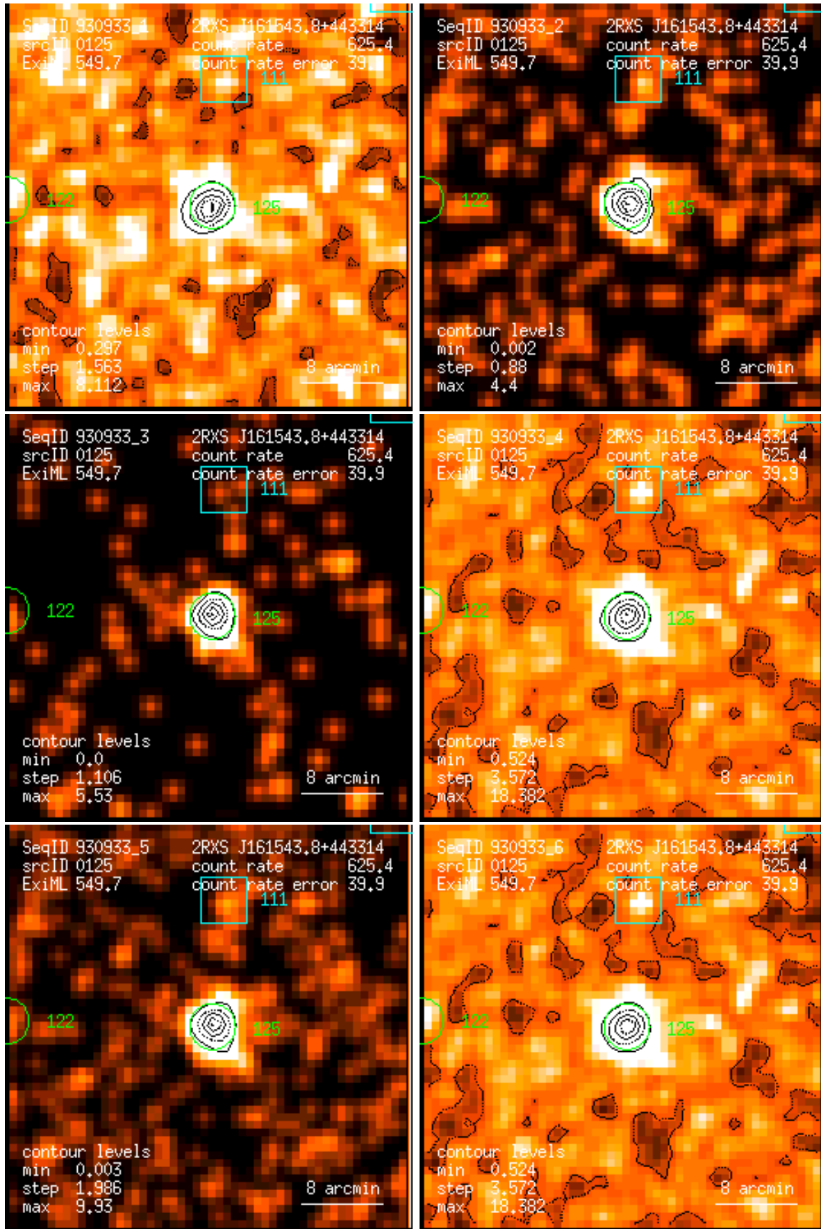
Figure 125: RASS 930933: detection 0125: band rate images, Gaussian filter: (1) PSPC channels 11 – 41, (2) 52 – 90, (3) 91 – 201, (4) 11 – 235, (5) 52 – 201, (6) 11 – 201. Broad band rates in counts/ks. Band rate contour levels in counts/ks/arcmin 2 .
