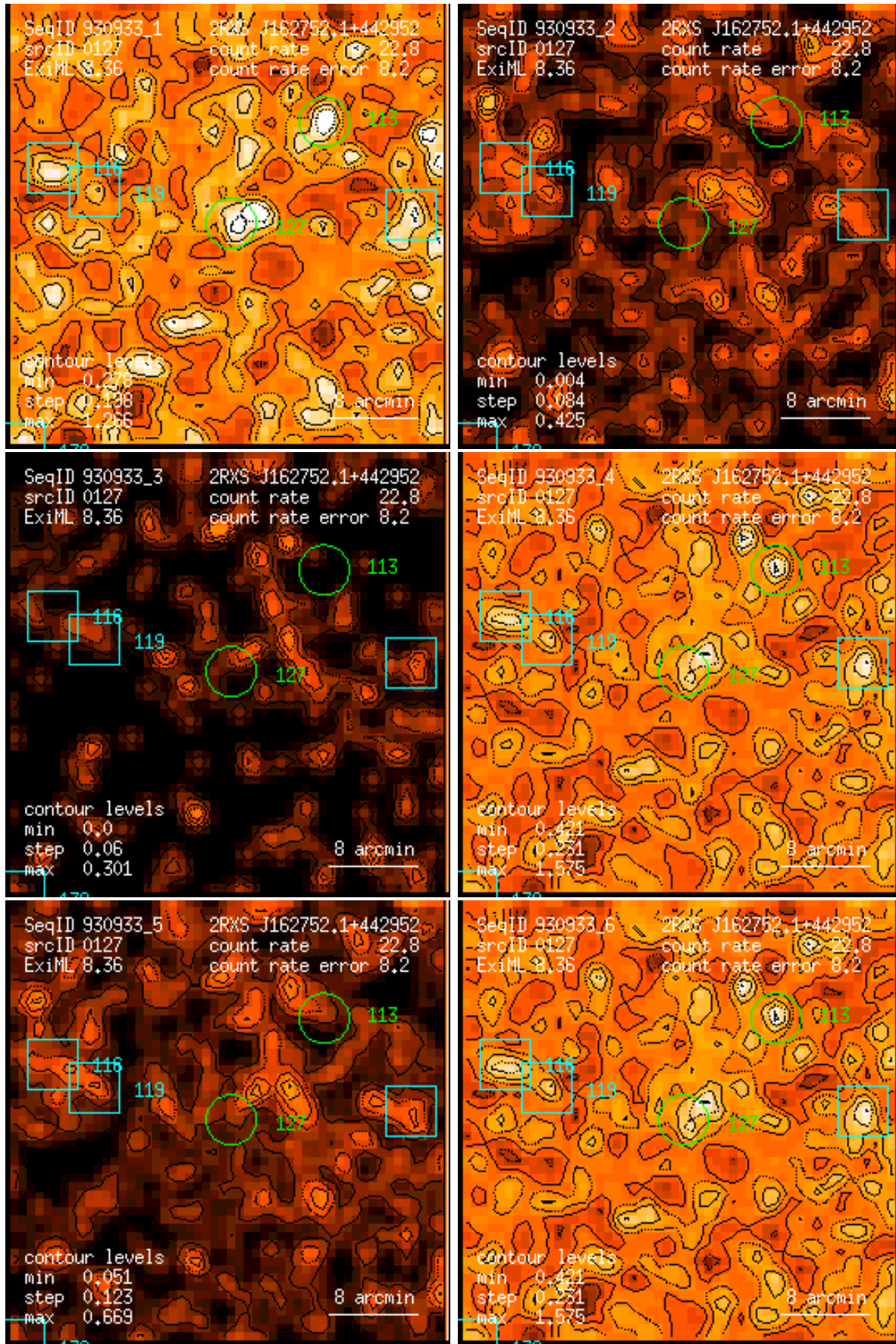
Figure 127: RASS 930933: detection 0127: band rate images, Gaussian filter: (1) PSPC channels 11 – 41, (2) 52 – 90, (3) 91 – 201, (4) 11 – 235, (5) 52 – 201, (6) 11 – 201. Broad band rates in counts/ks. Band rate contour levels in counts/ks/arcmin 2 .
