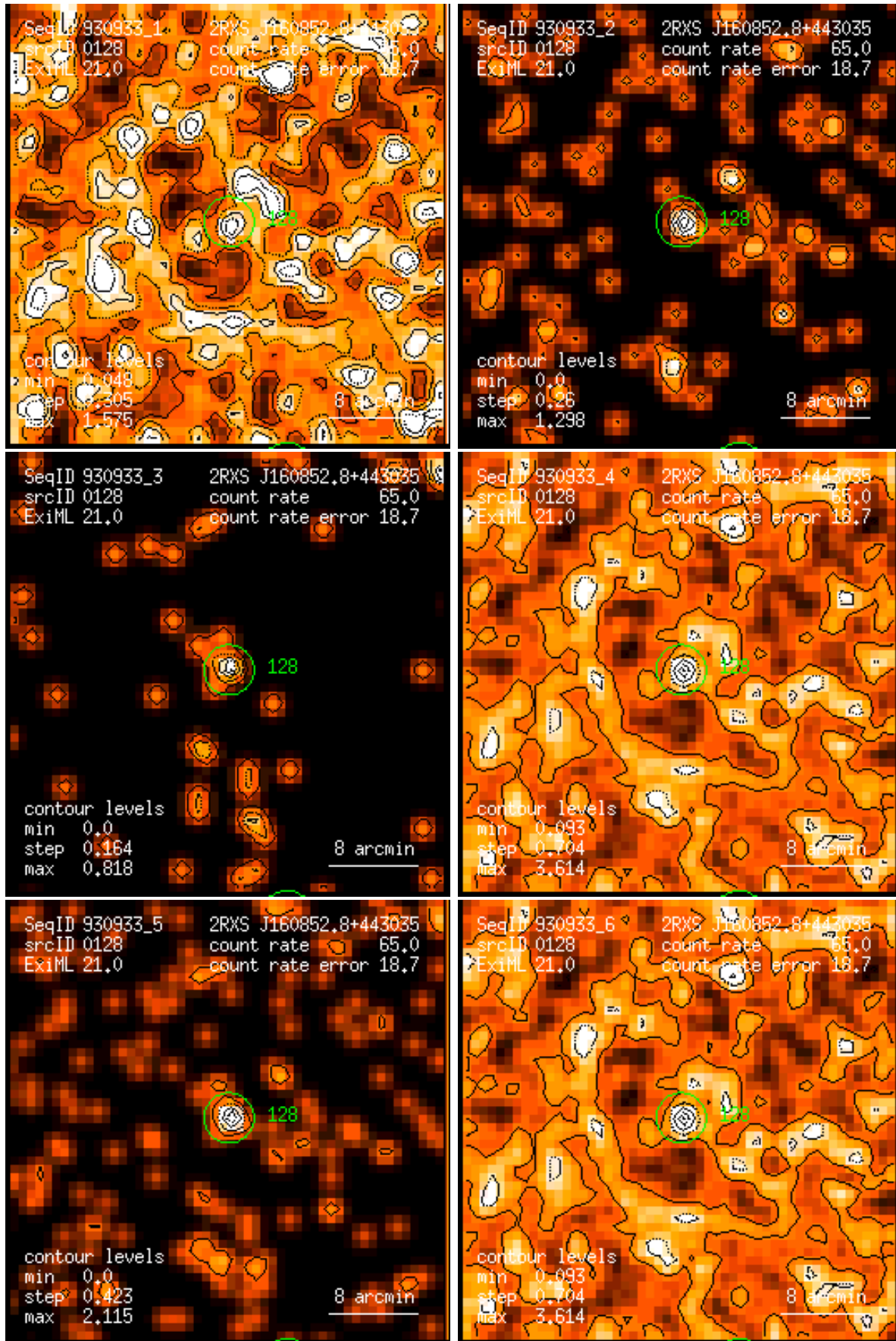
Figure 128: RASS 930933: detection 0128: band rate images, Gaussian filter: (1) PSPC channels 11 – 41, (2) 52 – 90, (3) 91 – 201, (4) 11 – 235, (5) 52 – 201, (6) 11 – 201. Broad band rates in counts/ks. Band rate contour levels in counts/ks/arcmin 2 .
