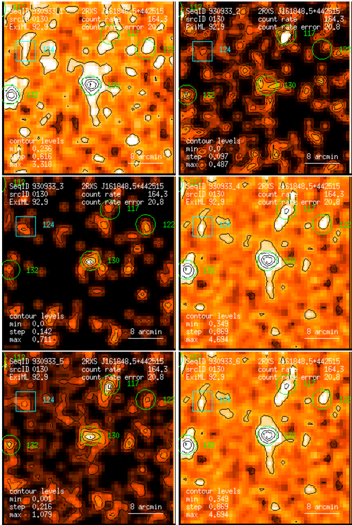
Figure 130: RASS 930933: detection 0130: band rate images, Gaussian filter: (1) PSPC channels 11 – 41, (2) 52 – 90, (3) 91 – 201, (4) 11 – 235, (5) 52 – 201, (6) 11 – 201. Broad band rates in counts/ks. Band rate contour levels in counts/ks/arcmin 2 .
