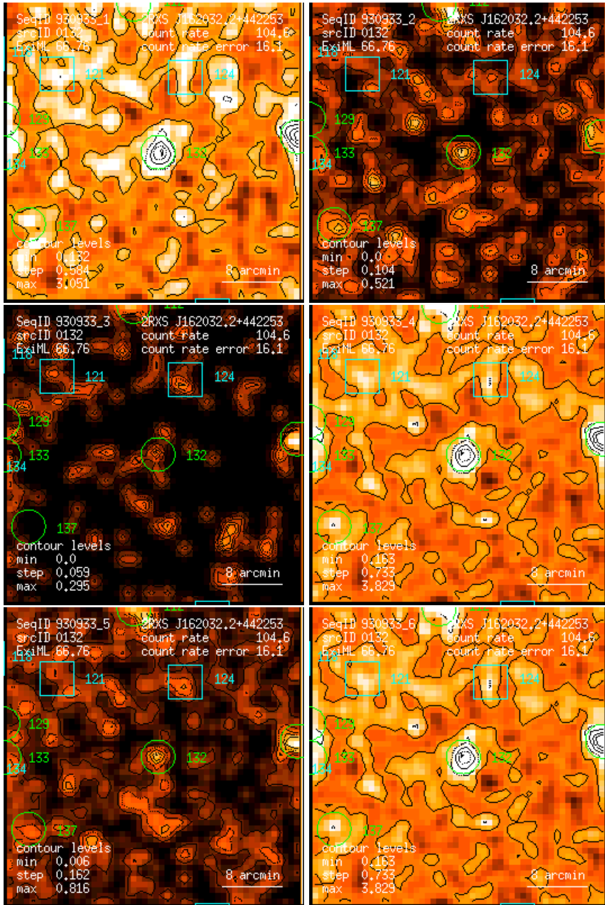
Figure 132: RASS 930933: detection 0132: band rate images, Gaussian filter: (1) PSPC channels 11 – 41, (2) 52 – 90, (3) 91 – 201, (4) 11 – 235, (5) 52 – 201, (6) 11 – 201. Broad band rates in counts/ks. Band rate contour levels in counts/ks/arcmin 2 .
