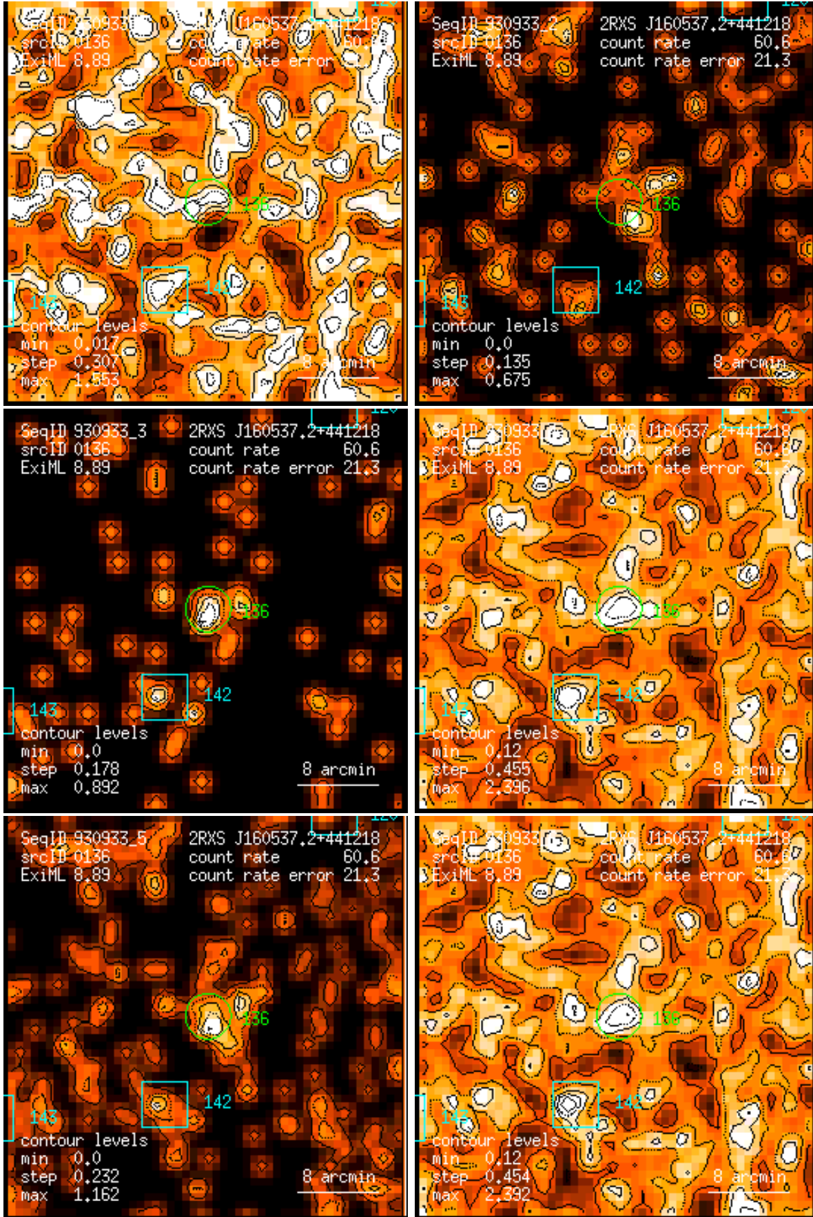
Figure 136: RASS 930933: detection 0136: band rate images, Gaussian filter: (1) PSPC channels 11 – 41, (2) 52 – 90, (3) 91 – 201, (4) 11 – 235, (5) 52 – 201, (6) 11 – 201. Broad band rates in counts/ks. Band rate contour levels in counts/ks/arcmin 2 .
