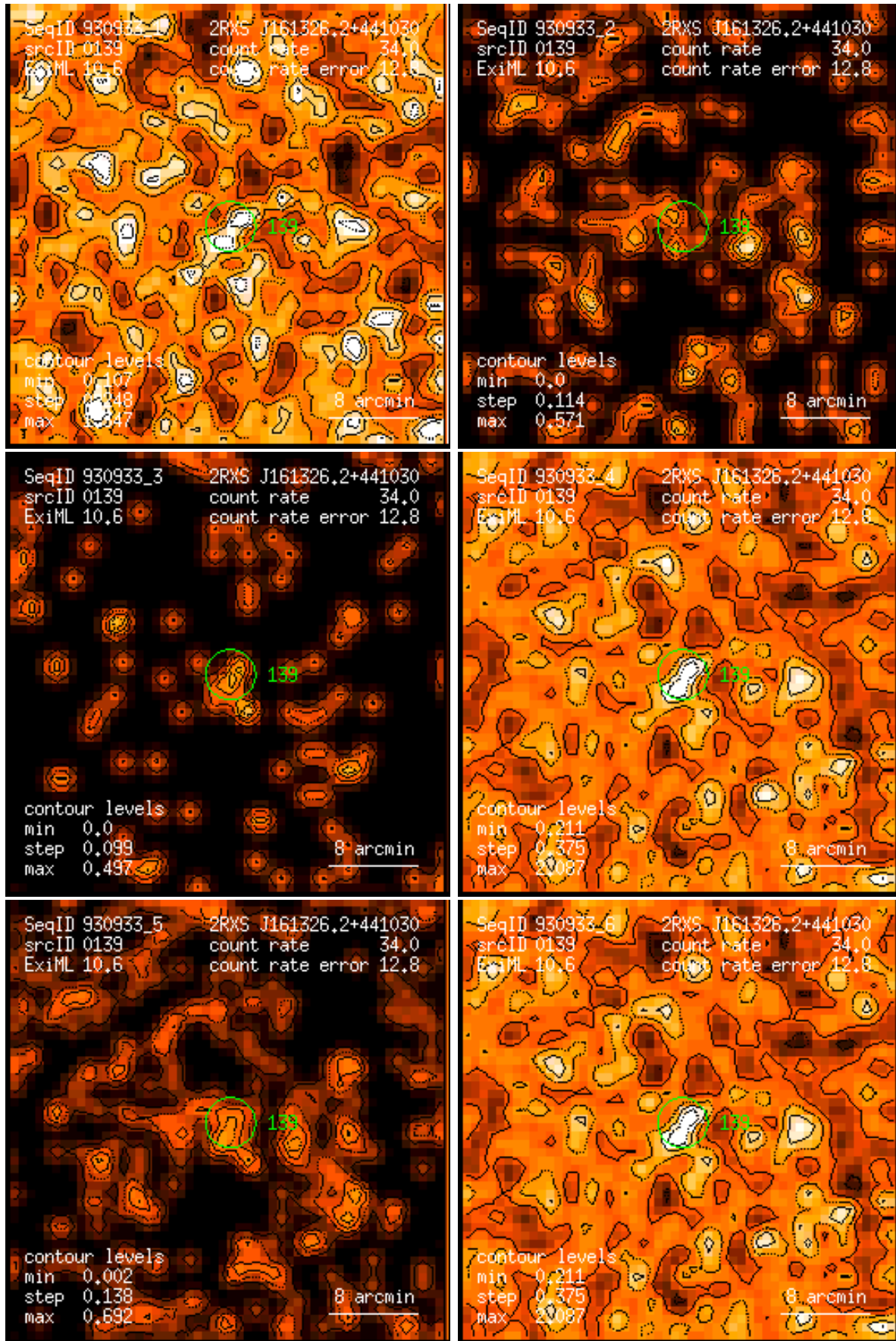
Figure 139: RASS 930933: detection 0139: band rate images, Gaussian filter: (1) PSPC channels 11 – 41, (2) 52 – 90, (3) 91 – 201, (4) 11 – 235, (5) 52 – 201, (6) 11 – 201. Broad band rates in counts/ks. Band rate contour levels in counts/ks/arcmin 2 .
