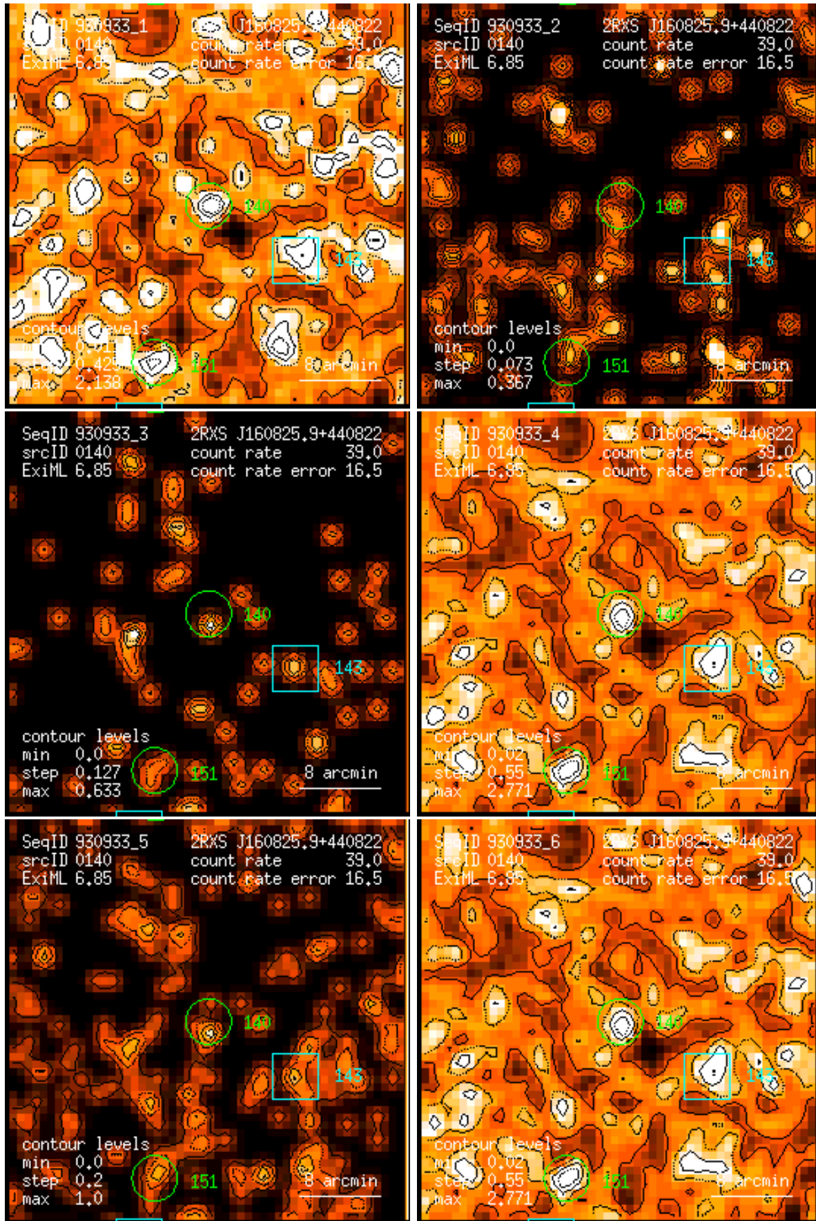
Figure 140: RASS 930933: detection 0140: band rate images, Gaussian filter: (1) PSPC channels 11 – 41, (2) 52 – 90, (3) 91 – 201, (4) 11 – 235, (5) 52 – 201, (6) 11 – 201. Broad band rates in counts/ks. Band rate contour levels in counts/ks/arcmin 2 .
