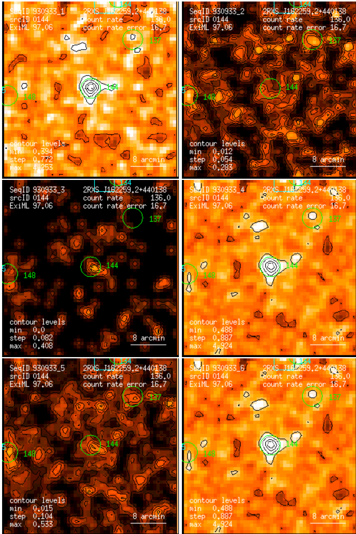
Figure 144: RASS 930933: detection 0144: band rate images, Gaussian filter: (1) PSPC channels 11 – 41, (2) 52 – 90, (3) 91 – 201, (4) 11 – 235, (5) 52 – 201, (6) 11 – 201. Broad band rates in counts/ks. Band rate contour levels in counts/ks/arcmin 2 .
