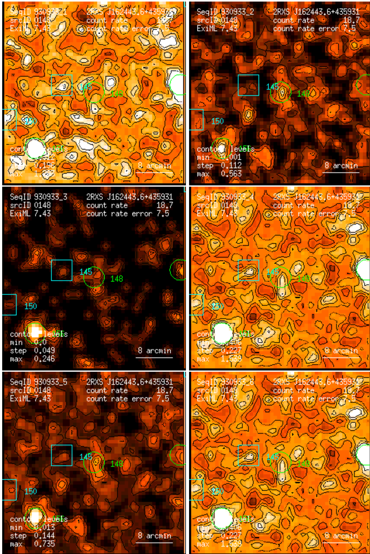
Figure 148: RASS 930933: detection 0148: band rate images, Gaussian filter: (1) PSPC channels 11 – 41, (2) 52 – 90, (3) 91 – 201, (4) 11 – 235, (5) 52 – 201, (6) 11 – 201. Broad band rates in counts/ks. Band rate contour levels in counts/ks/arcmin 2 .
