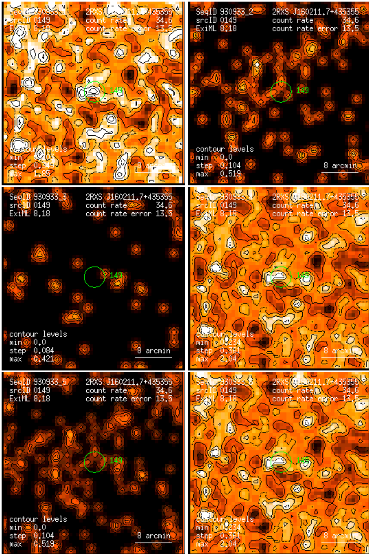
Figure 149: RASS 930933: detection 0149: band rate images, Gaussian filter: (1) PSPC channels 11 – 41, (2) 52 – 90, (3) 91 – 201, (4) 11 – 235, (5) 52 – 201, (6) 11 – 201. Broad band rates in counts/ks. Band rate contour levels in counts/ks/arcmin 2 .
