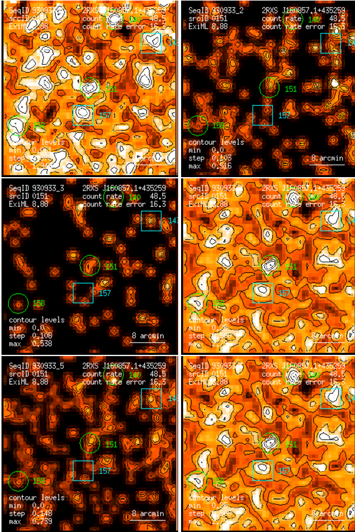
Figure 151: RASS 930933: detection 0151: band rate images, Gaussian filter: (1) PSPC channels 11 – 41, (2) 52 – 90, (3) 91 – 201, (4) 11 – 235, (5) 52 – 201, (6) 11 – 201. Broad band rates in counts/ks. Band rate contour levels in counts/ks/arcmin 2 .
