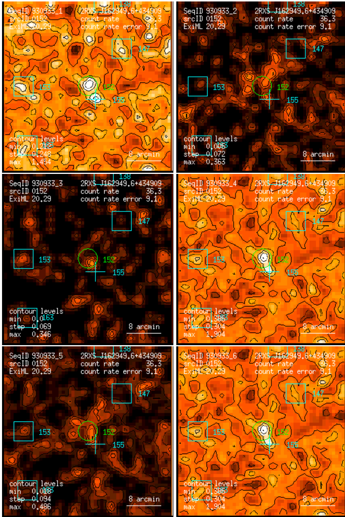
Figure 152: RASS 930933: detection 0152: band rate images, Gaussian filter: (1) PSPC channels 11 – 41, (2) 52 – 90, (3) 91 – 201, (4) 11 – 235, (5) 52 – 201, (6) 11 – 201. Broad band rates in counts/ks. Band rate contour levels in counts/ks/arcmin 2 .
