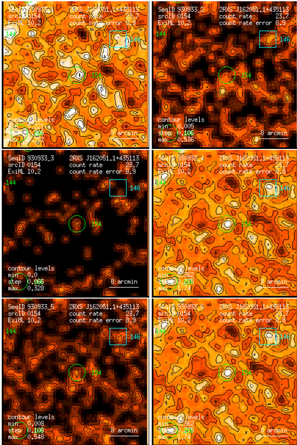
Figure 154: RASS 930933: detection 0154: band rate images, Gaussian filter: (1) PSPC channels 11 – 41, (2) 52 – 90, (3) 91 – 201, (4) 11 – 235, (5) 52 – 201, (6) 11 – 201. Broad band rates in counts/ks. Band rate contour levels in counts/ks/arcmin 2 .
