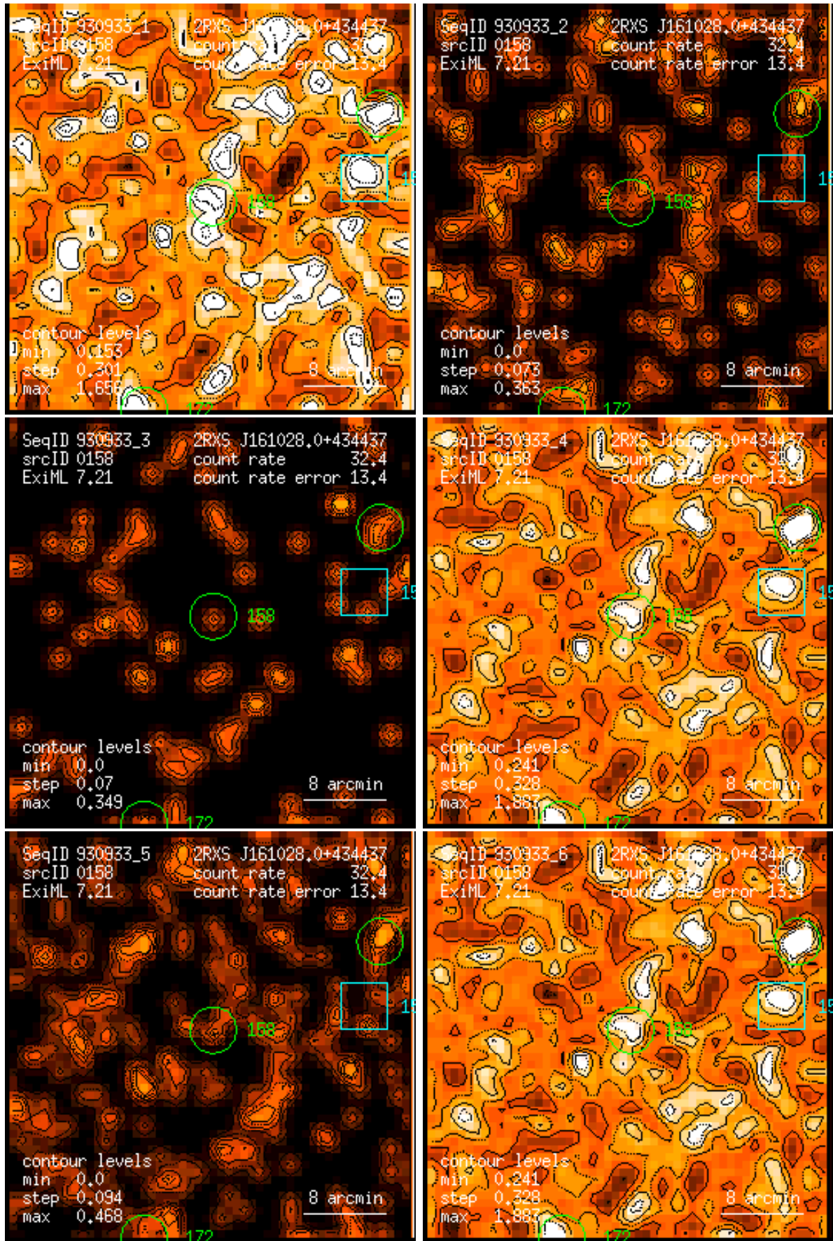
Figure 158: RASS 930933: detection 0158: band rate images, Gaussian filter: (1) PSPC channels 11 – 41, (2) 52 – 90, (3) 91 – 201, (4) 11 – 235, (5) 52 – 201, (6) 11 – 201. Broad band rates in counts/ks. Band rate contour levels in counts/ks/arcmin 2 .
