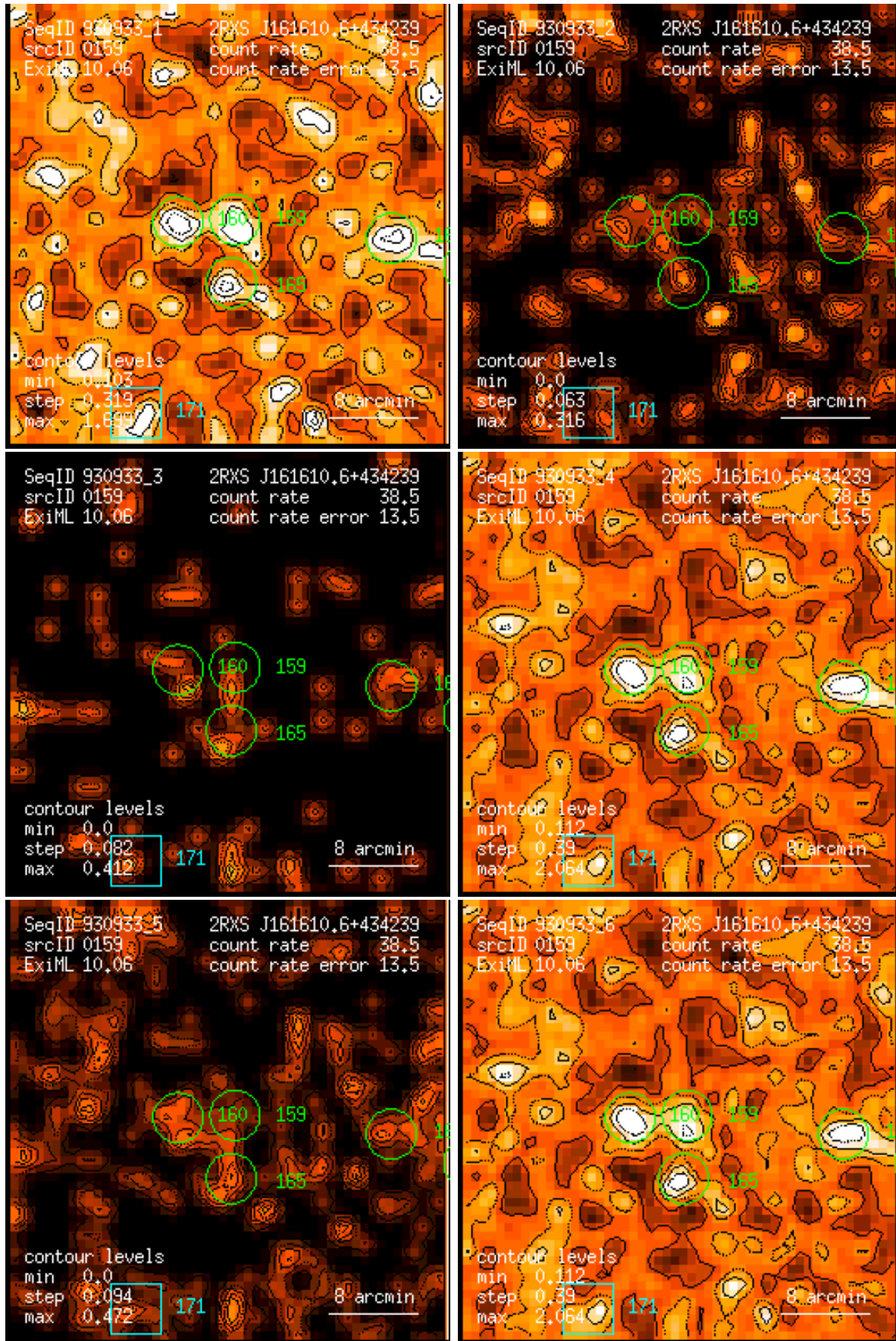
Figure 159: RASS 930933: detection 0159: band rate images, Gaussian filter: (1) PSPC channels 11 – 41, (2) 52 – 90, (3) 91 – 201, (4) 11 – 235, (5) 52 – 201, (6) 11 – 201. Broad band rates in counts/ks. Band rate contour levels in counts/ks/arcmin 2 .
