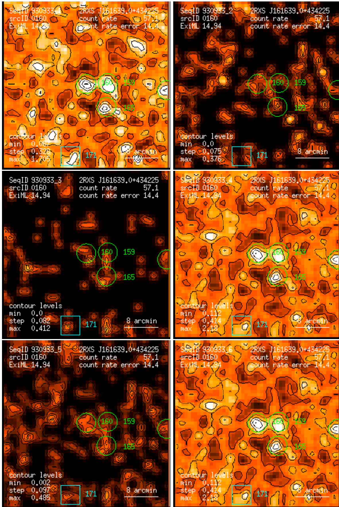
Figure 160: RASS 930933: detection 0160: band rate images, Gaussian filter: (1) PSPC channels 11 – 41, (2) 52 – 90, (3) 91 – 201, (4) 11 – 235, (5) 52 – 201, (6) 11 – 201. Broad band rates in counts/ks. Band rate contour levels in counts/ks/arcmin 2 .
