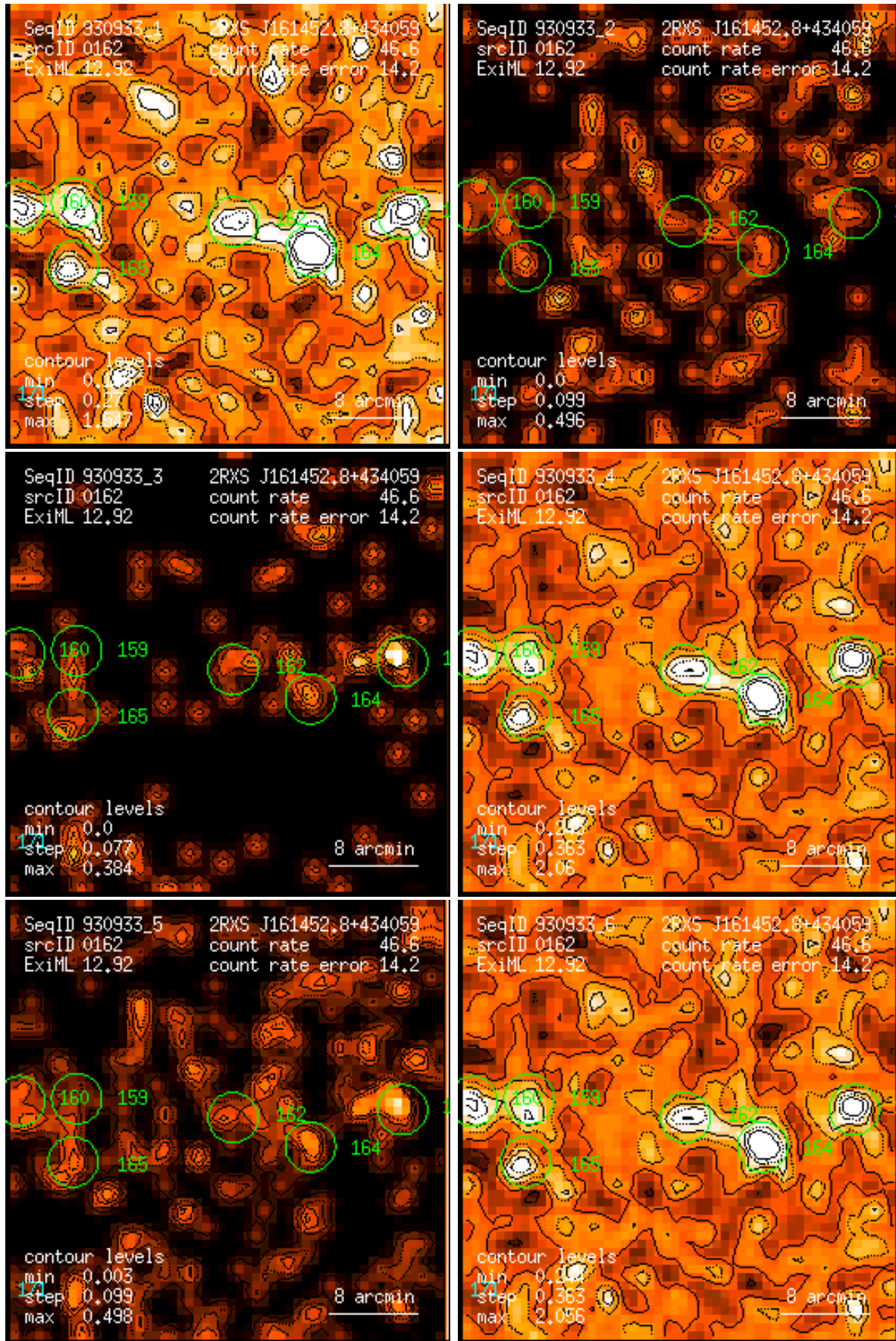
Figure 162: RASS 930933: detection 0162: band rate images, Gaussian filter: (1) PSPC channels 11 – 41, (2) 52 – 90, (3) 91 – 201, (4) 11 – 235, (5) 52 – 201, (6) 11 – 201. Broad band rates in counts/ks. Band rate contour levels in counts/ks/arcmin 2 .
