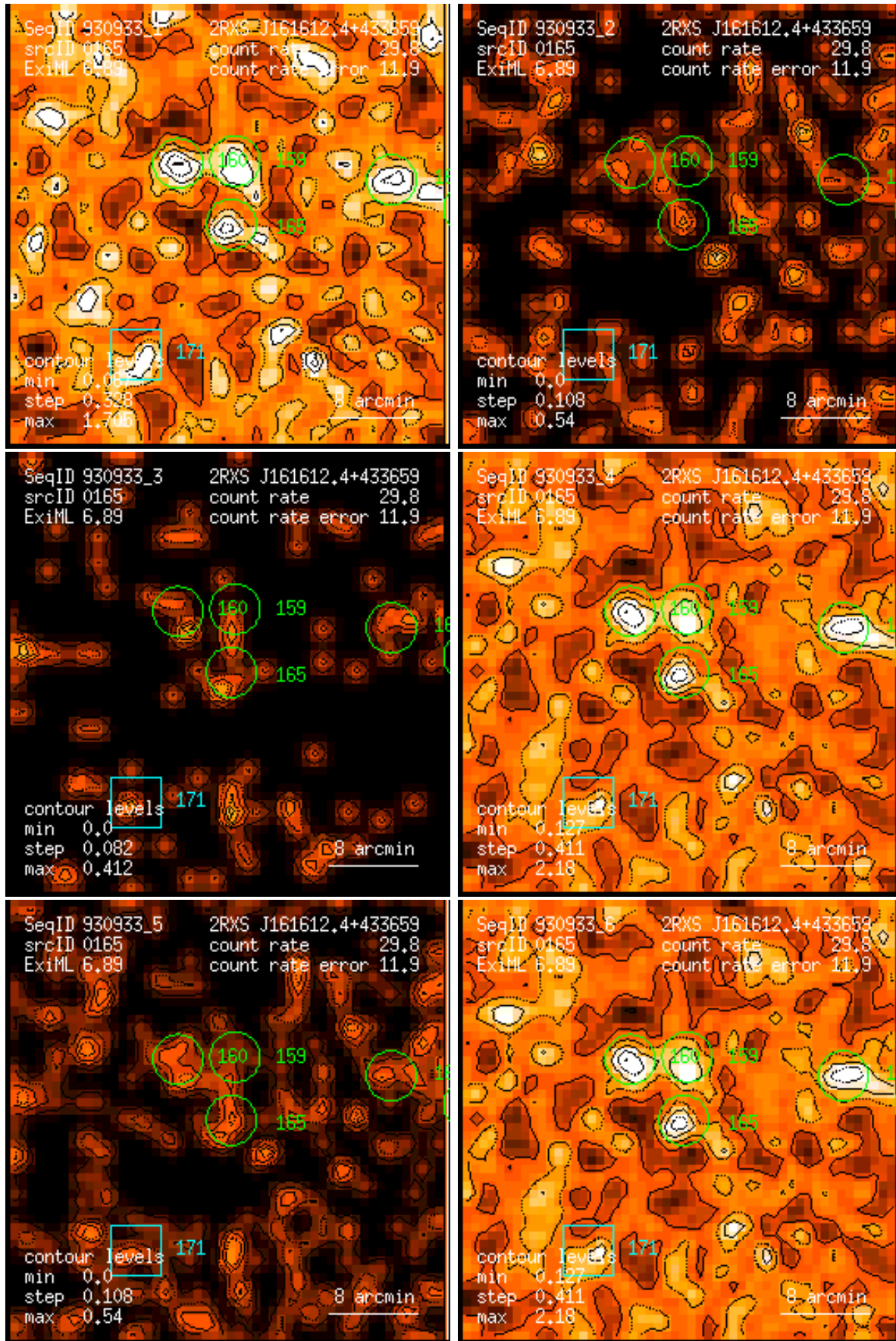
Figure 165: RASS 930933: detection 0165: band rate images, Gaussian filter: (1) PSPC channels 11 – 41, (2) 52 – 90, (3) 91 – 201, (4) 11 – 235, (5) 52 – 201, (6) 11 – 201. Broad band rates in counts/ks. Band rate contour levels in counts/ks/arcmin 2 .
