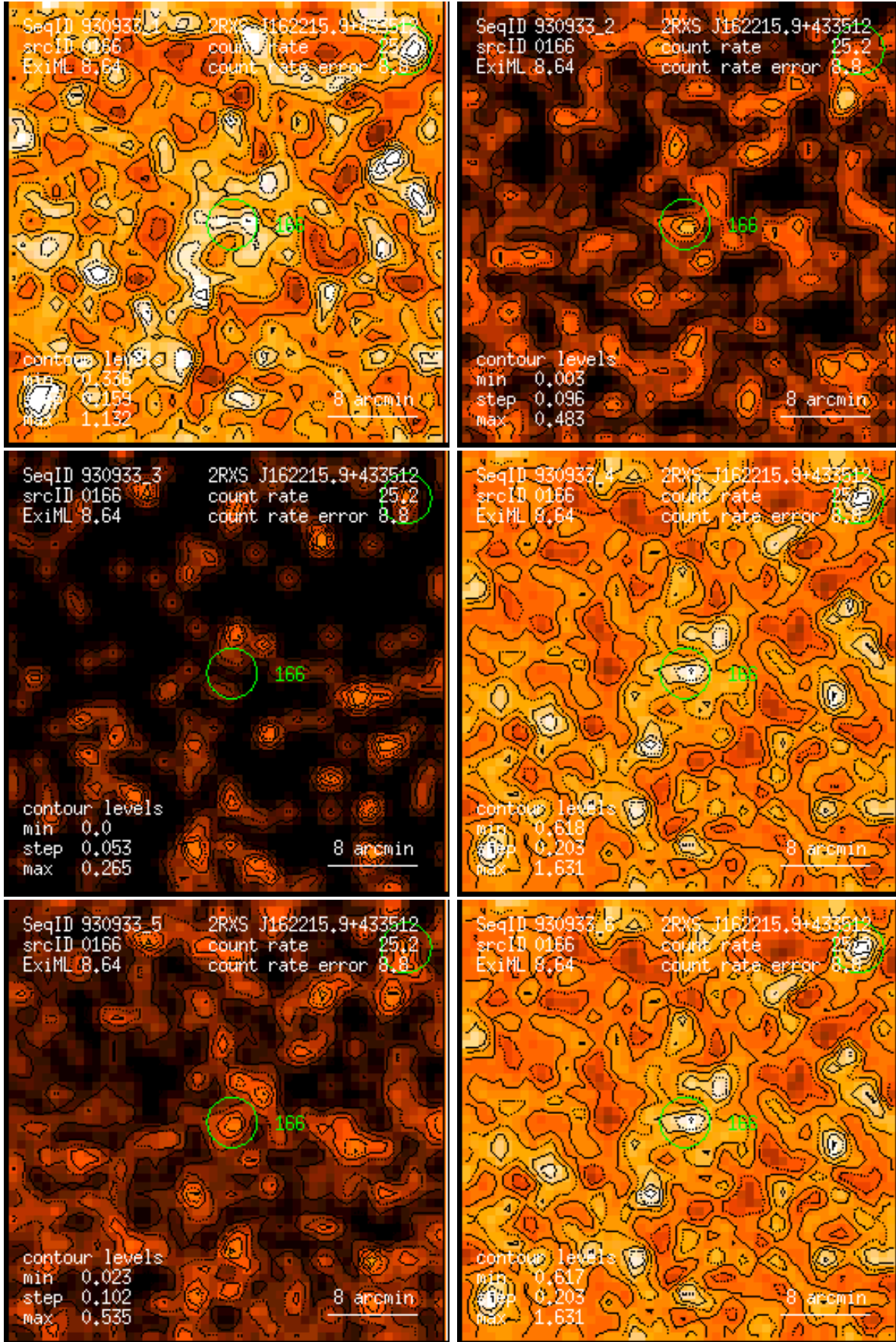
Figure 166: RASS 930933: detection 0166: band rate images, Gaussian filter: (1) PSPPC channels 11 – 41, (2) 52 – 90, (3) 91 – 201, (4) 11 – 235, (5) 52 – 201, (6) 11 – 201. Broad band rates in counts/ks. Band rate contour levels in counts/ks/arcmin 2 .
