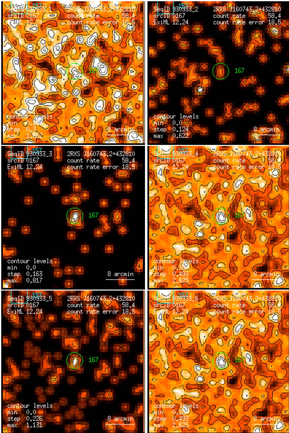
Figure 167: RASS 930933: detection 0167: band rate images, Gaussian filter: (1) PSPC channels 11 – 41, (2) 52 – 90, (3) 91 – 201, (4) 11 – 235, (5) 52 – 201, (6) 11 – 201. Broad band rates in counts/ks. Band rate contour levels in counts/ks/arcmin 2 .
