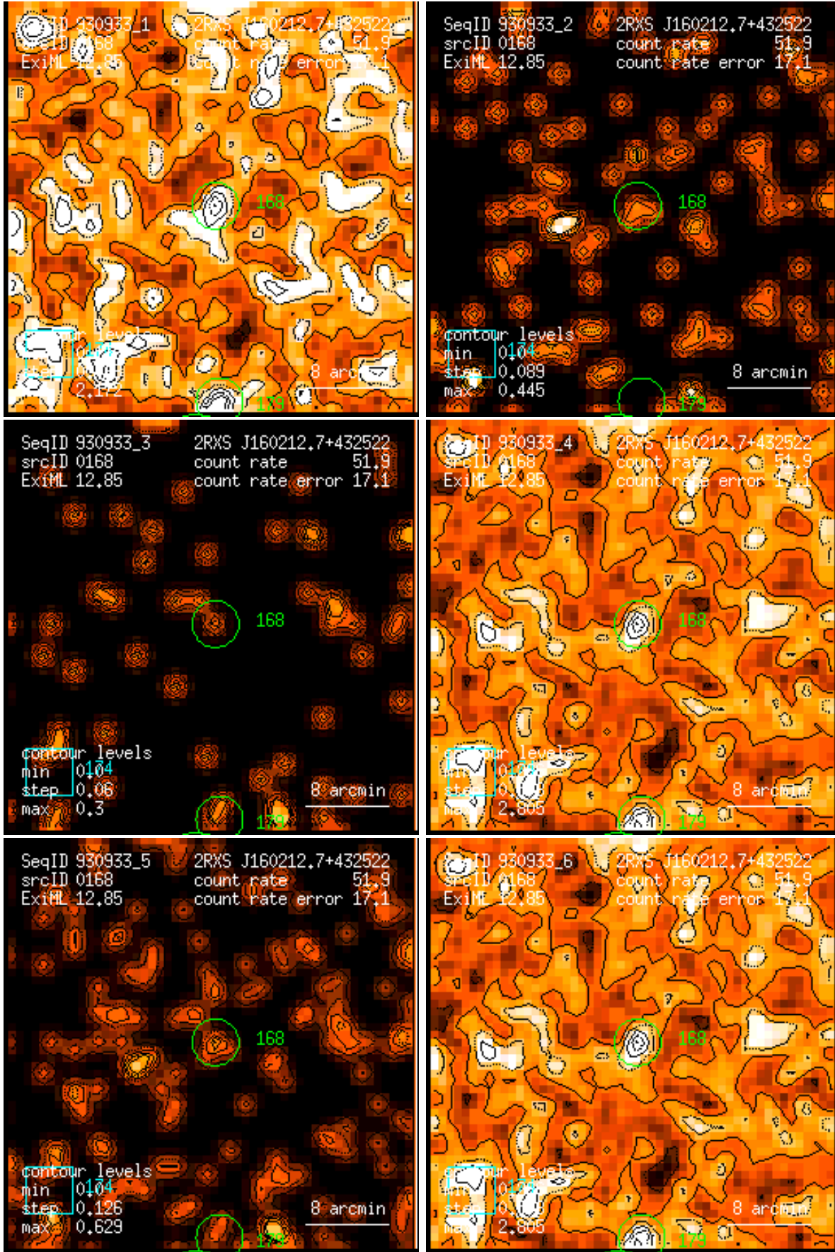
Figure 168: RASS 930933: detection 0168: band rate images, Gaussian filter: (1) PSPC channels 11 – 41, (2) 52 – 90, (3) 91 – 201, (4) 11 – 235, (5) 52 – 201, (6) 11 – 201. Broad band rates in counts/ks. Band rate contour levels in counts/ks/arcmin 2 .
