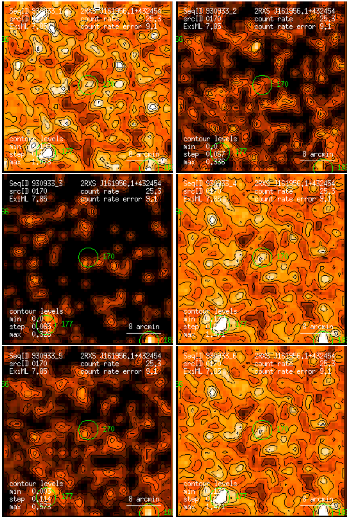
Figure 170: RASS 930933: detection 0170: band rate images, Gaussian filter: (1) PSPC channels 11 – 41, (2) 52 – 90, (3) 91 – 201, (4) 11 – 235, (5) 52 – 201, (6) 11 – 201. Broad band rates in counts/ks. Band rate contour levels in counts/ks/arcmin 2 .
