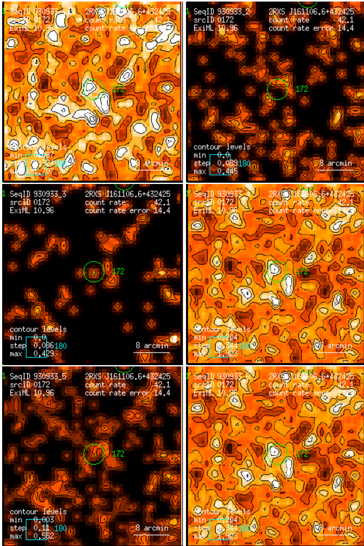
Figure 172: RASS 930933: detection 0172: band rate images, Gaussian filter: (1) PSPC channels 11 – 41, (2) 52 – 90, (3) 91 – 201, (4) 11 – 235, (5) 52 – 201, (6) 11 – 201. Broad band rates in counts/ks. Band rate contour levels in counts/ks/arcmin 2 .
