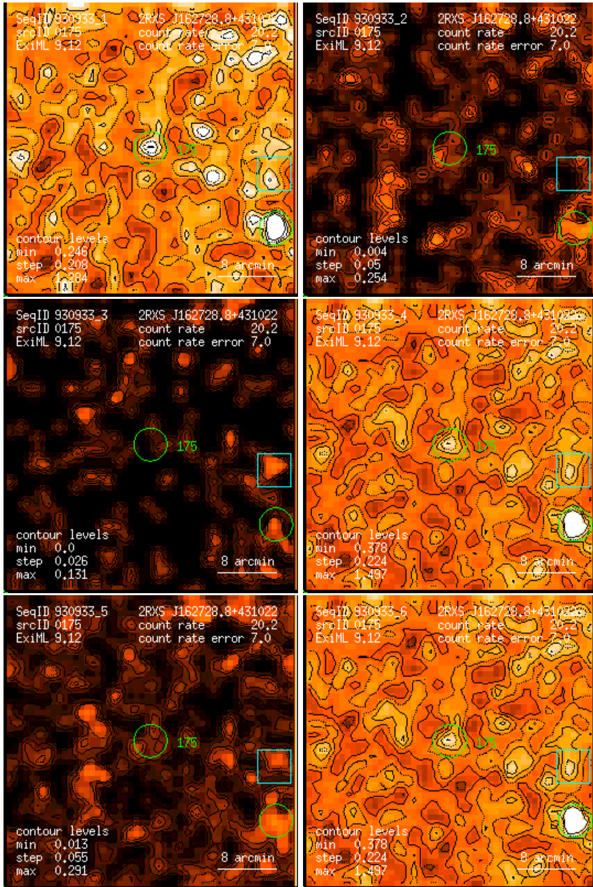
Figure 175: RASS 930933: detection 0175: band rate images, Gaussian filter: (1) PSPC channels 11 – 41, (2) 52 – 90, (3) 91 – 201, (4) 11 – 235, (5) 52 – 201, (6) 11 – 201. Broad band rates in counts/ks. Band rate contour levels in counts/ks/arcmin 2 .
